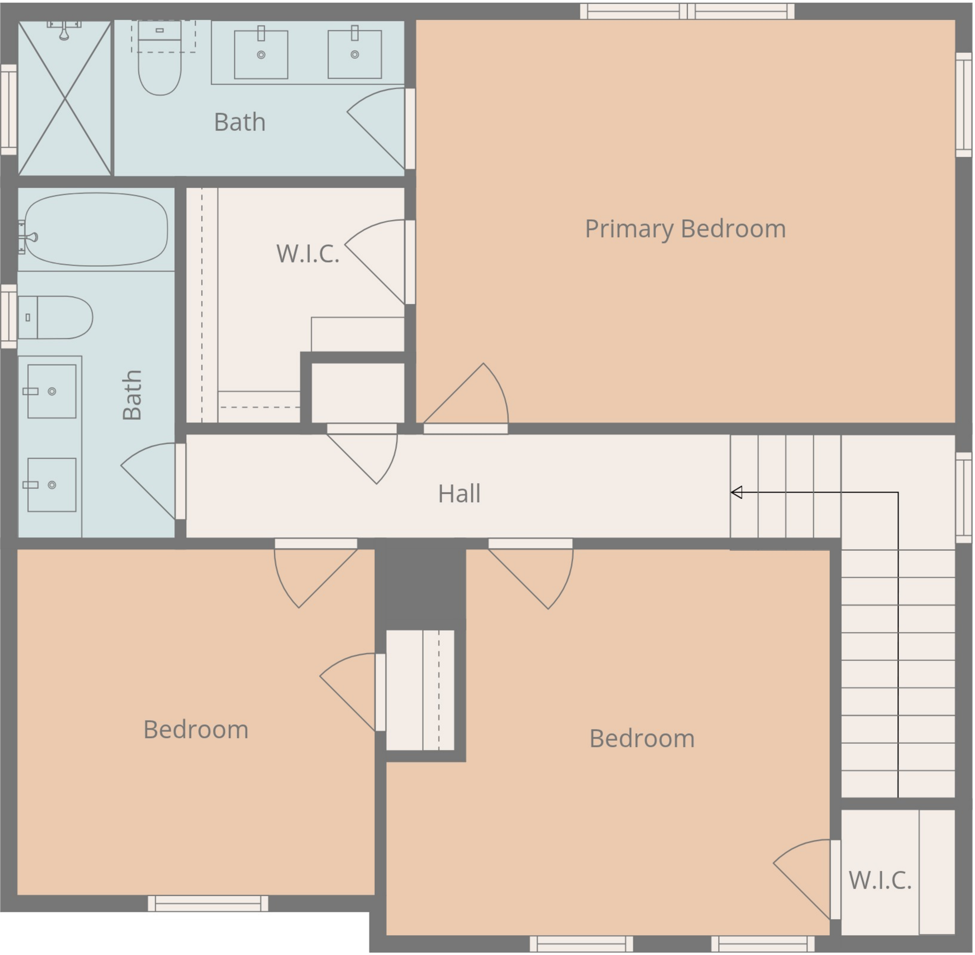
2nd Floor
