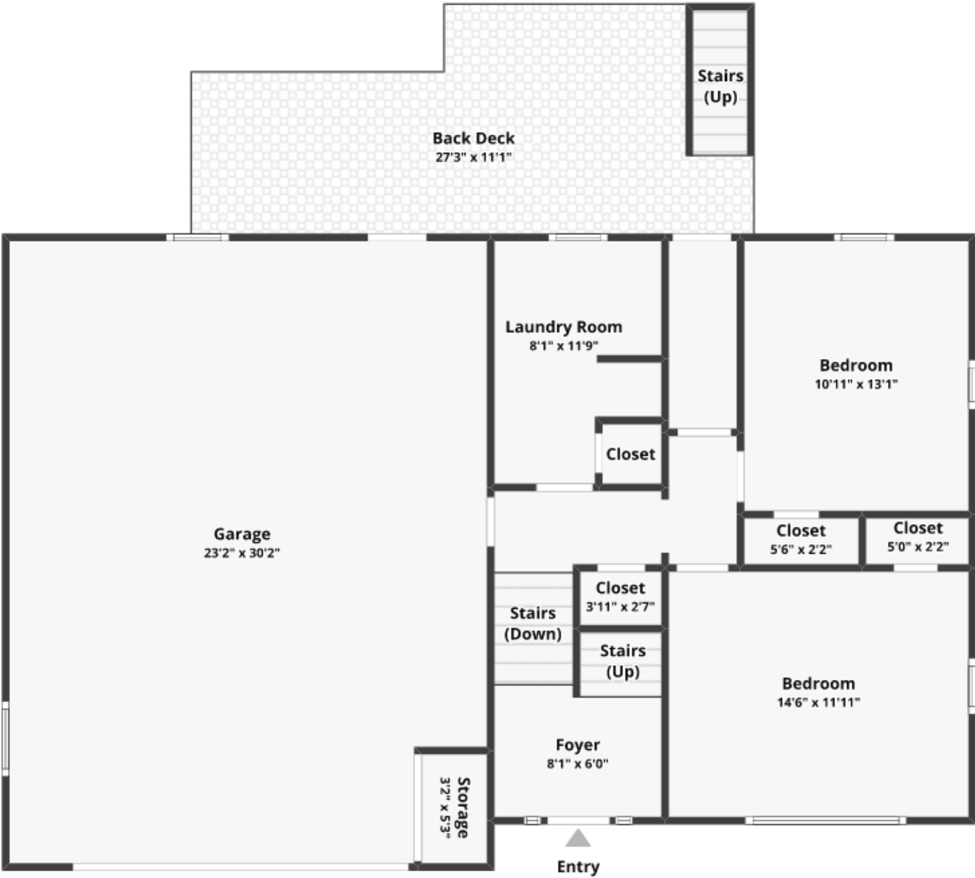
FLOOR 1 Finished area: ~606.49 sq. ft.
