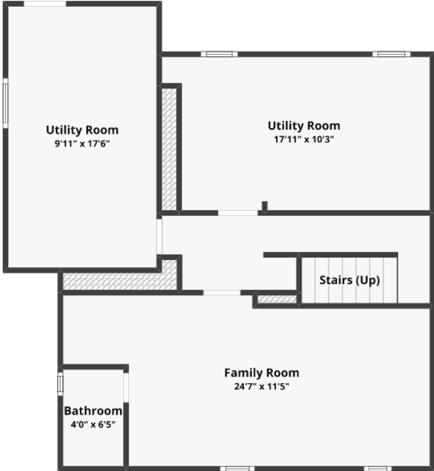
BASEMENT Finished area: ~681.07 sq. ft. Unfinished area: ~18.54 sq. ft.
