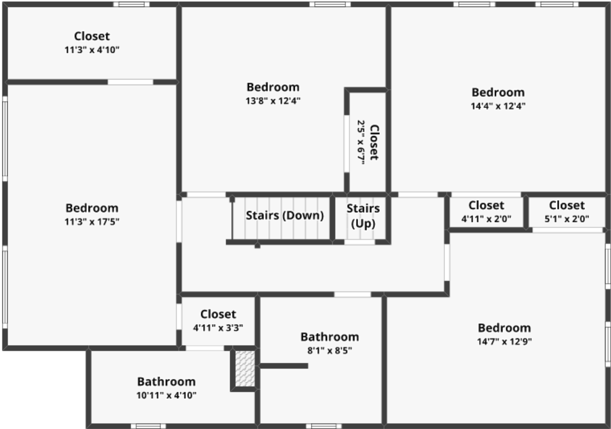
FLOOR 2 Finished area: ~1,007.63 sq. ft. Unfinished area: ~3.06 sq. ft.
