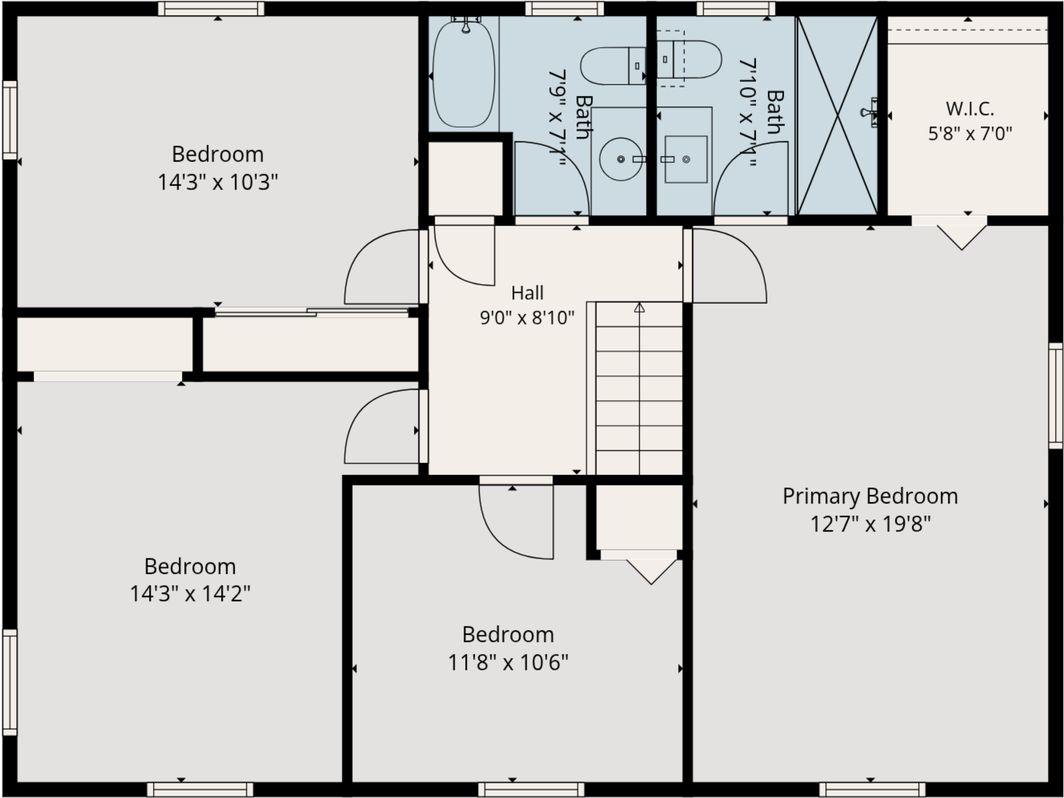
2nd Floor
