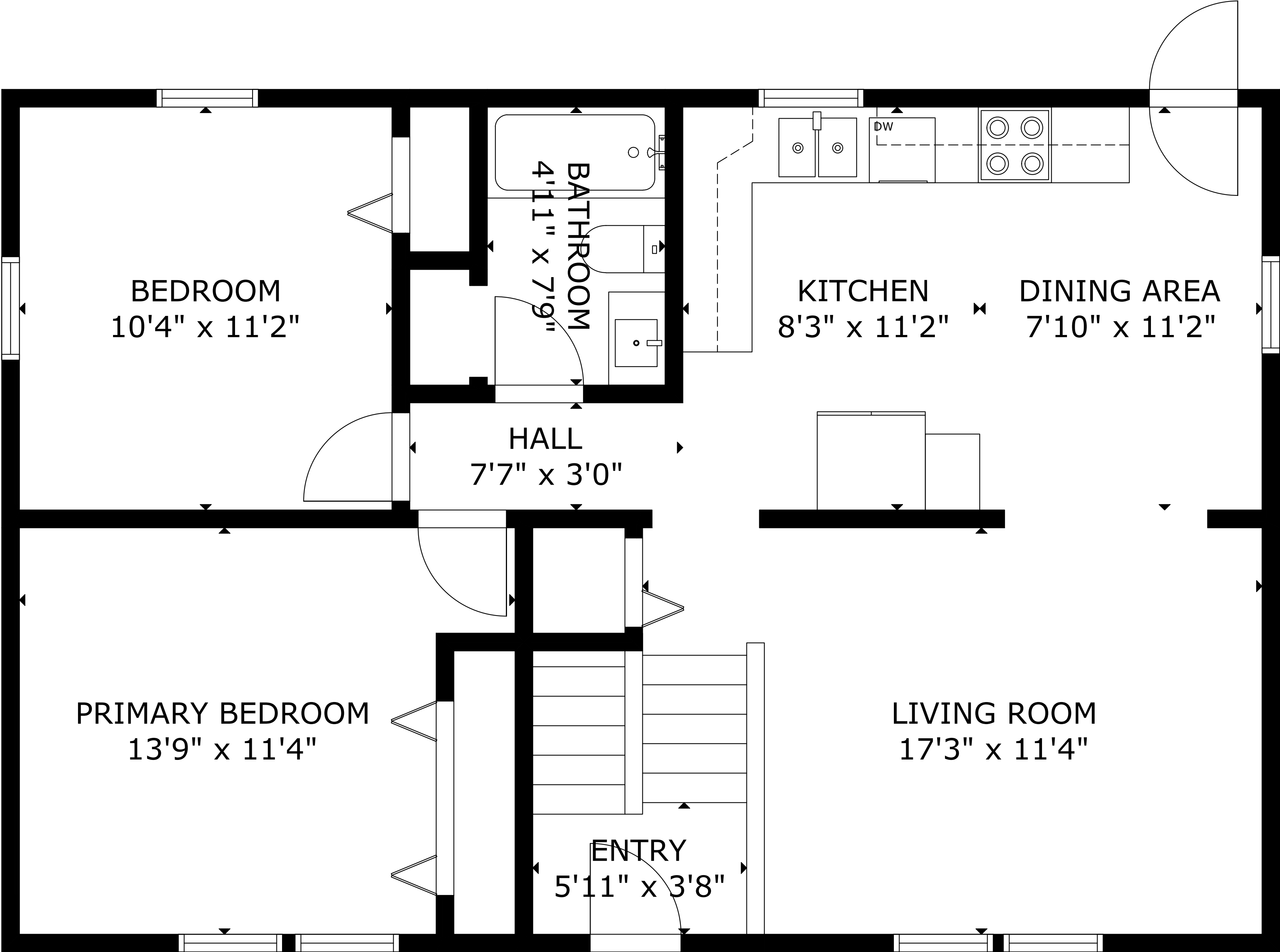
MAIN FLOOR
