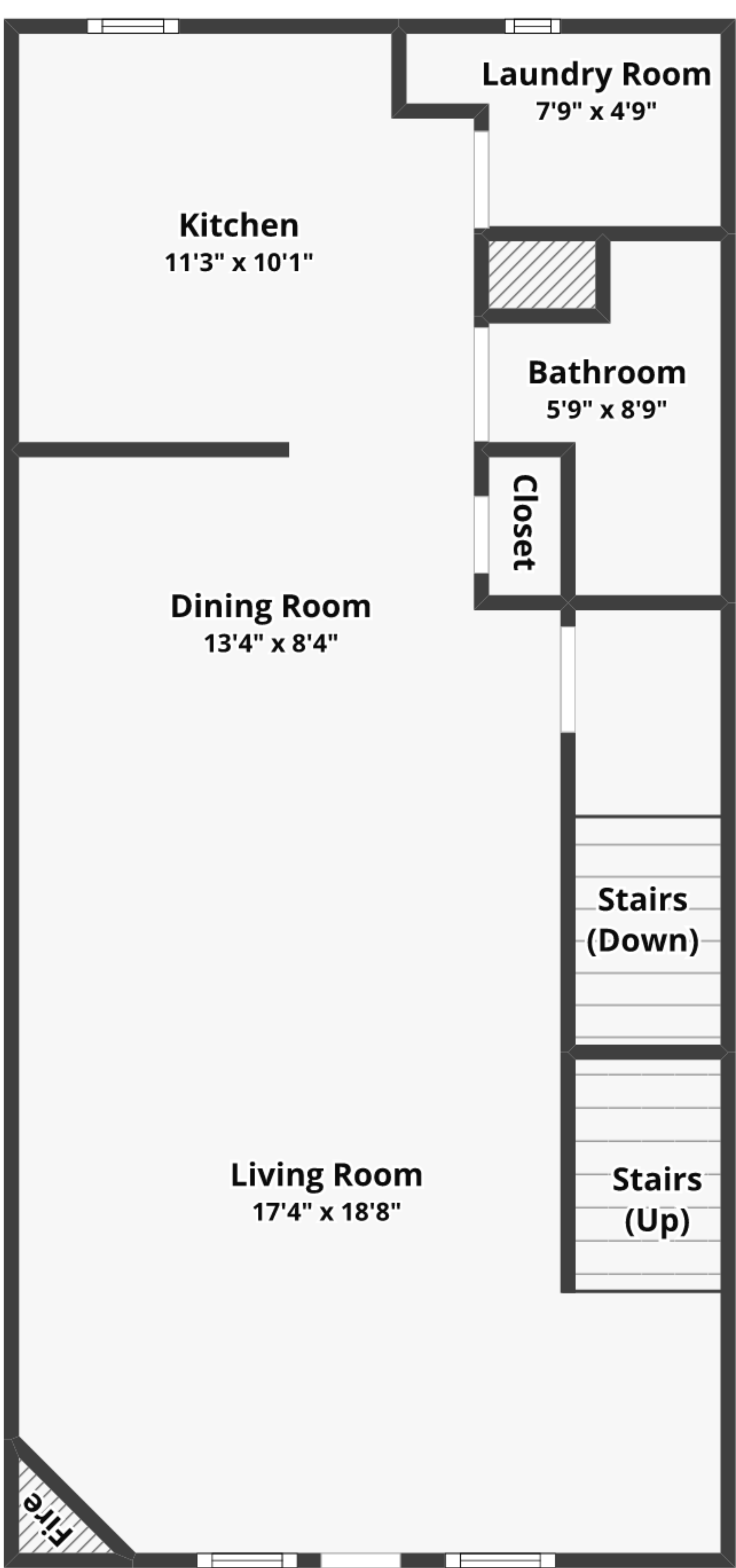
FLOOR 2
