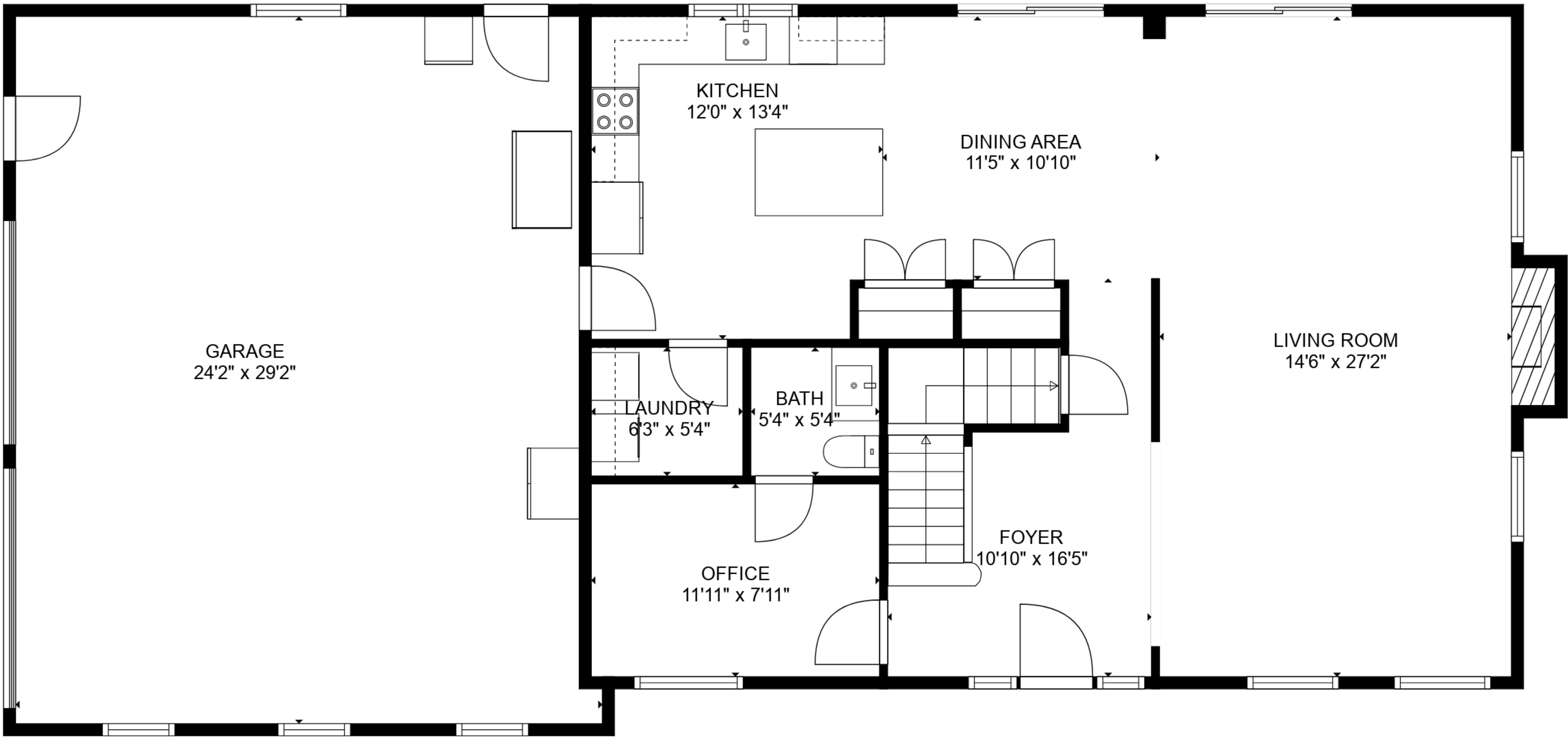
FLOOR 2
