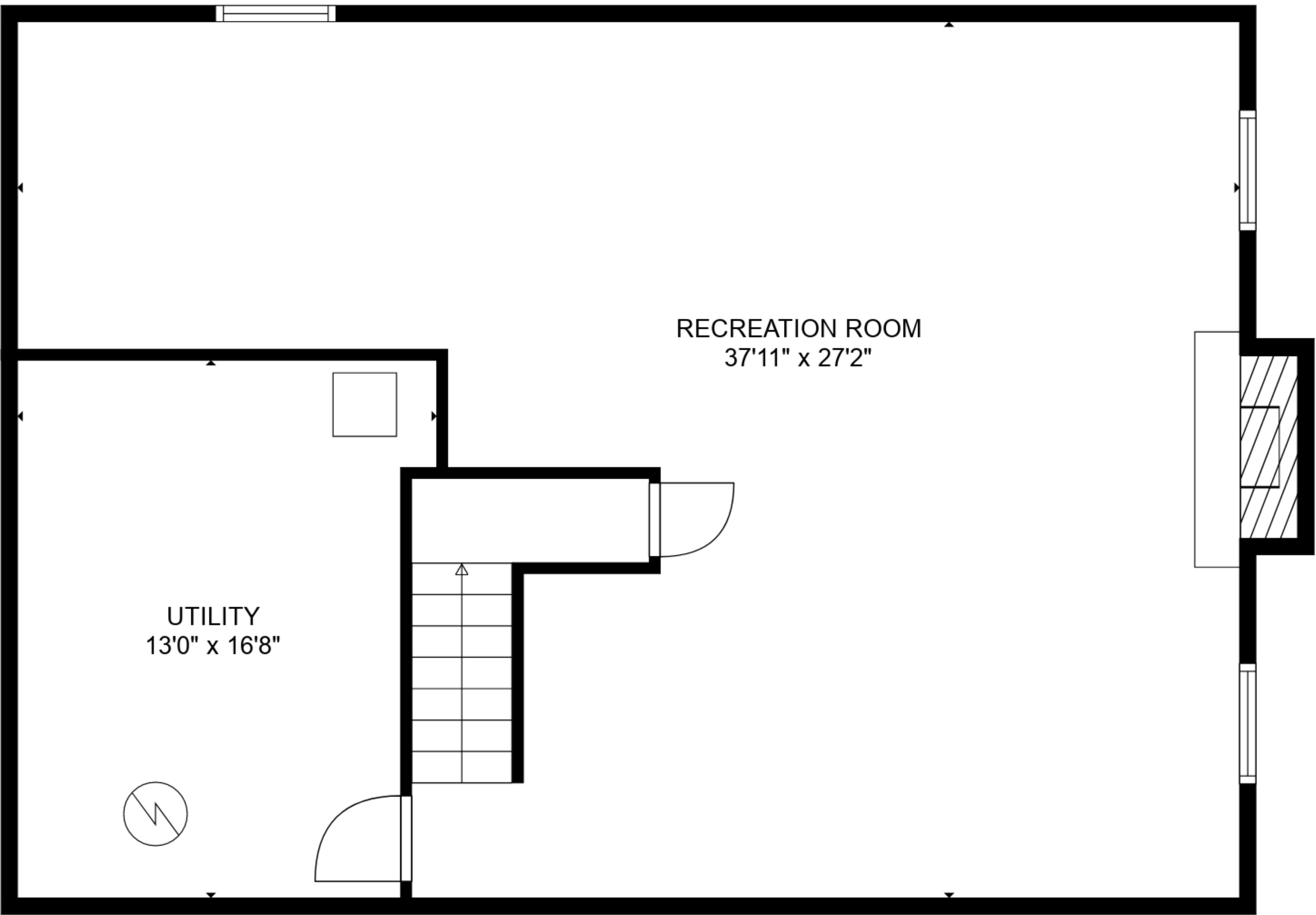
FLOOR 1
