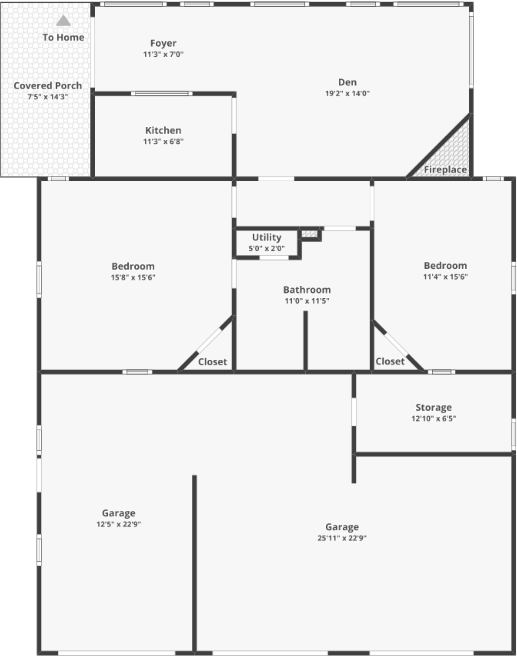
DETACHED BUNKHOUSE Finished area: ~1,068.29 sq. ft. Unfinished area: ~11.78 sq. ft.
