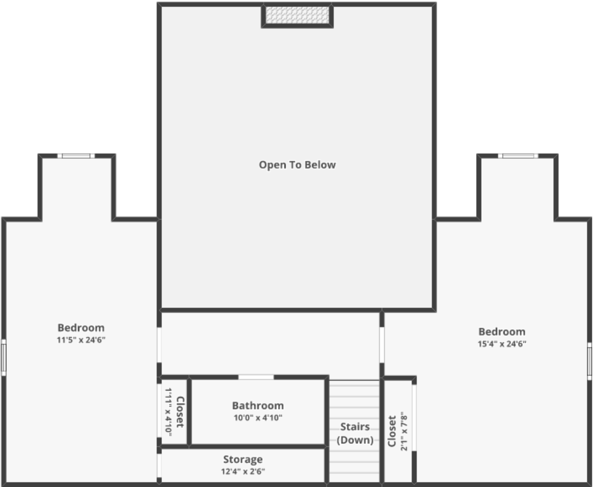
FLOOR 2 Finished area: ~743.22 sq. ft. Unfinished area: ~5.97 sq. ft.
