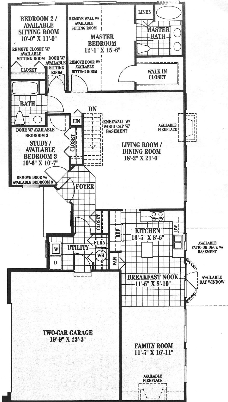
FIRST FLOOR PLAN WINDOW LOCATIONS VARY PER ELEVATION
