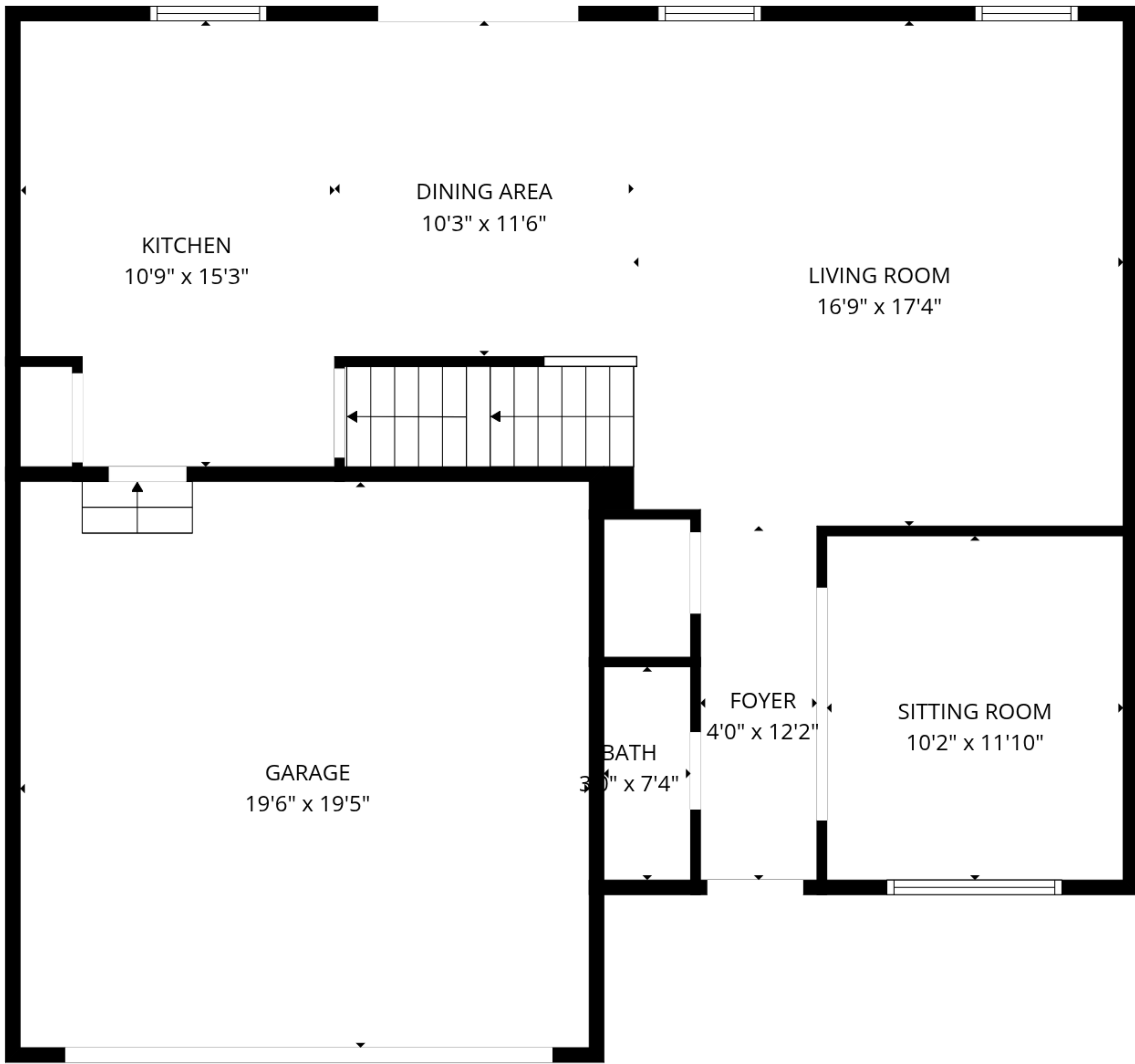
1st floor
