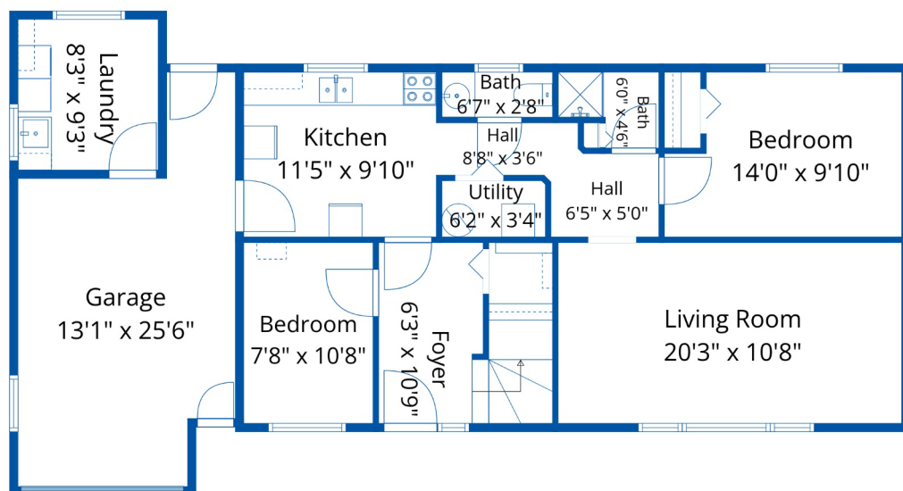
Below Main
