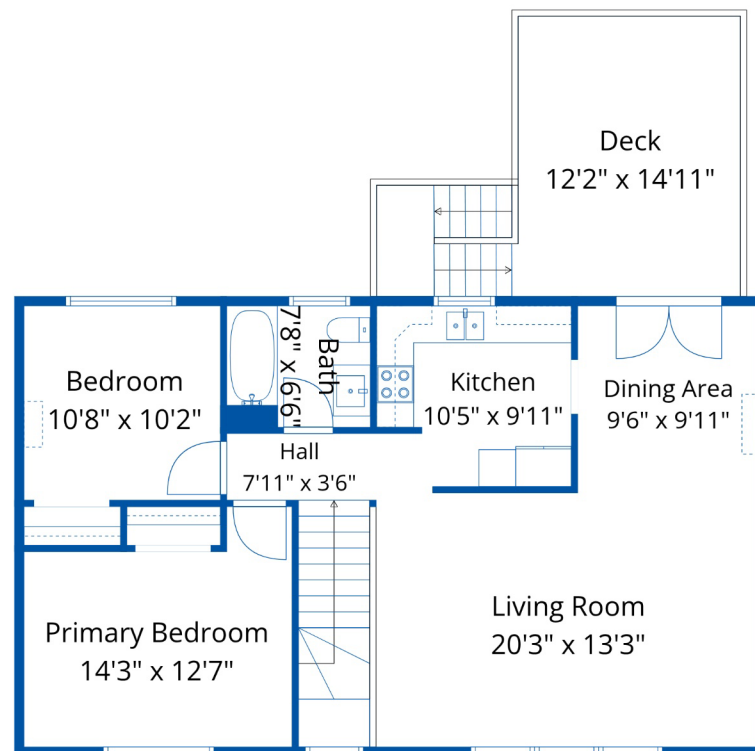
Main Floor
