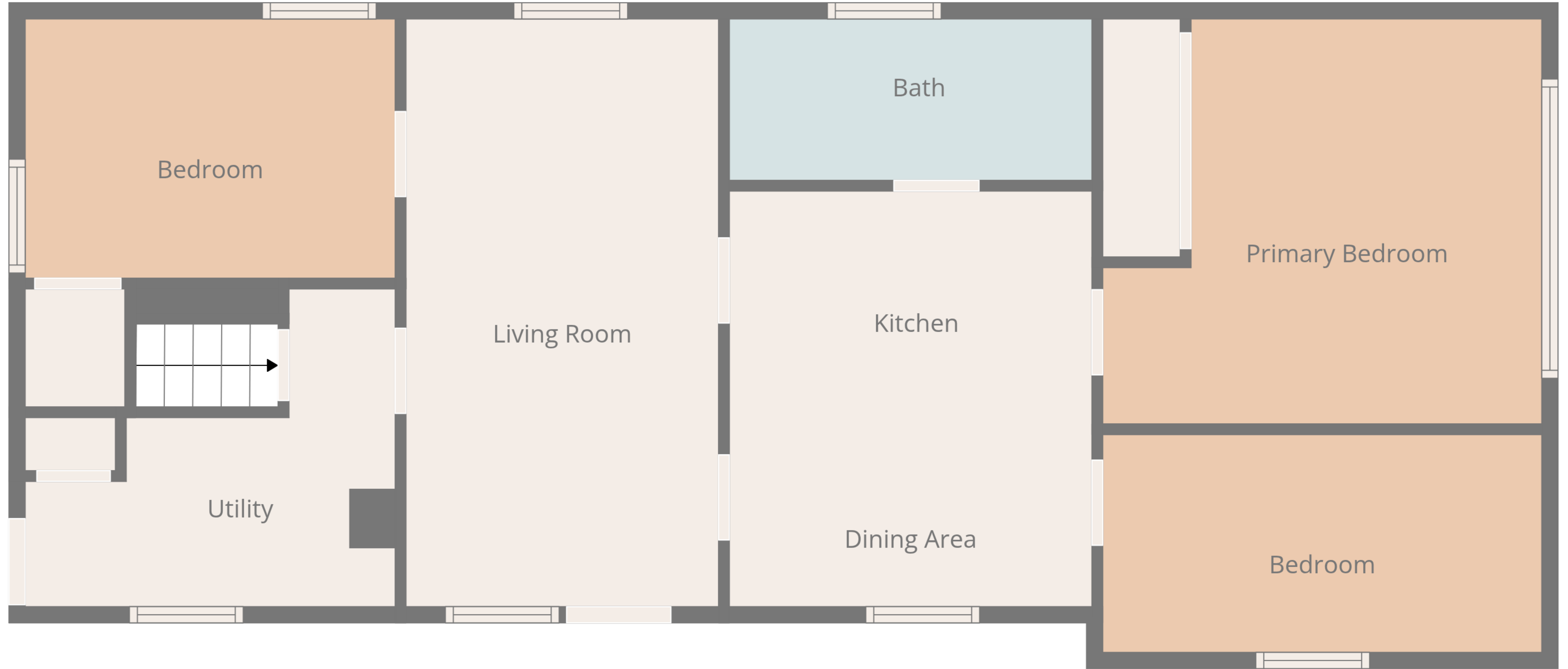
1st Floor
