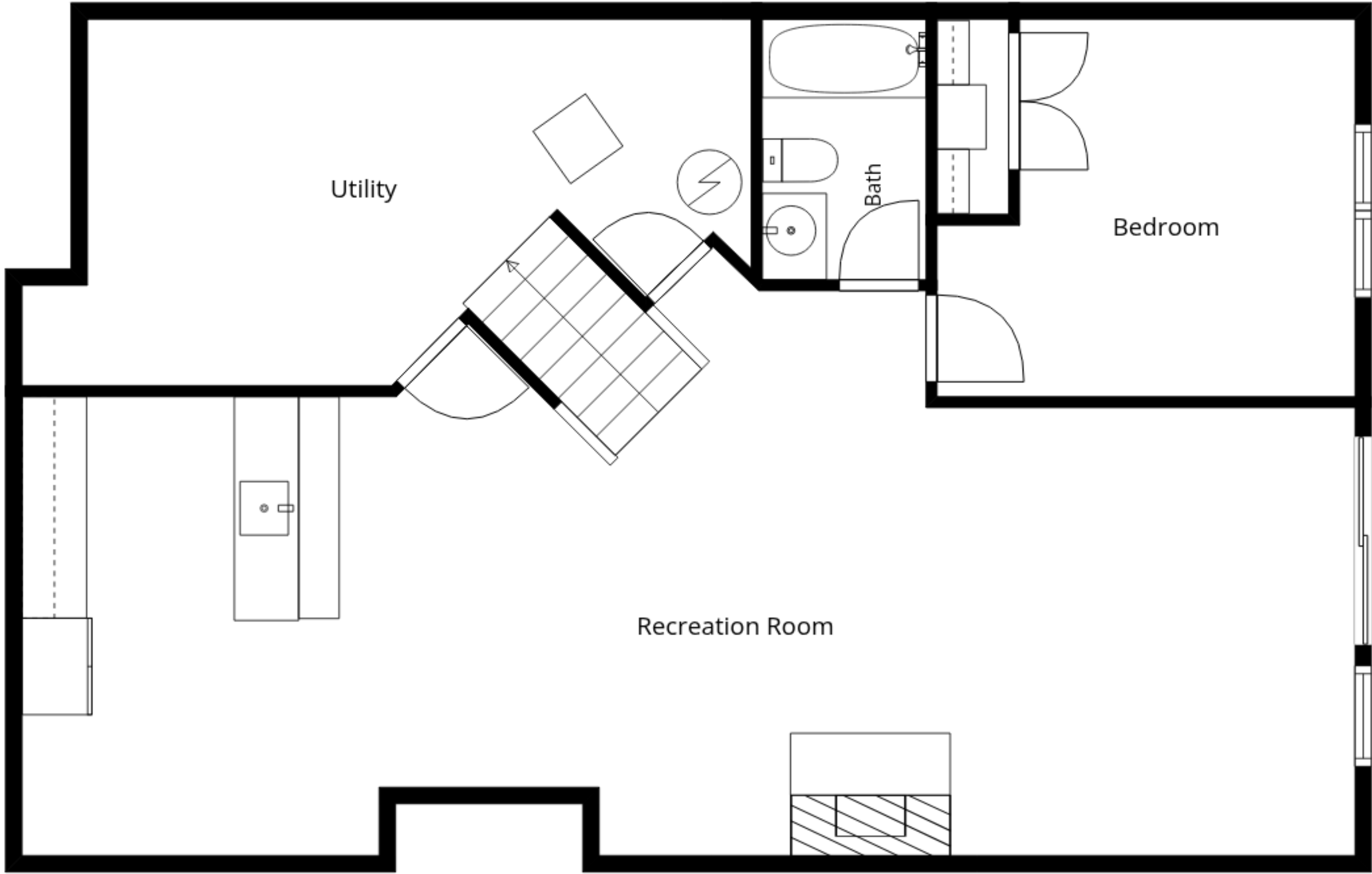
Basement
