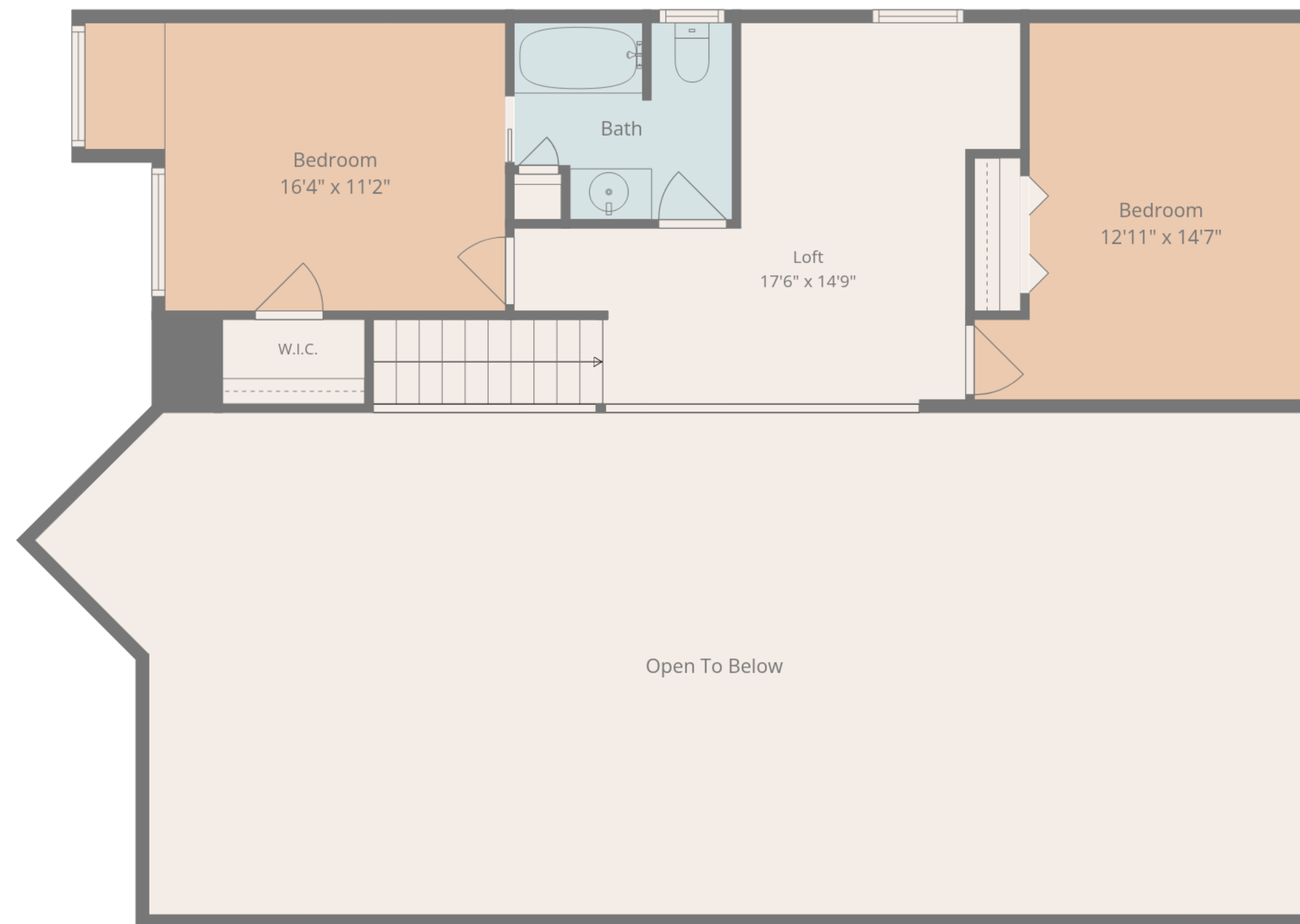
2nd Floor
