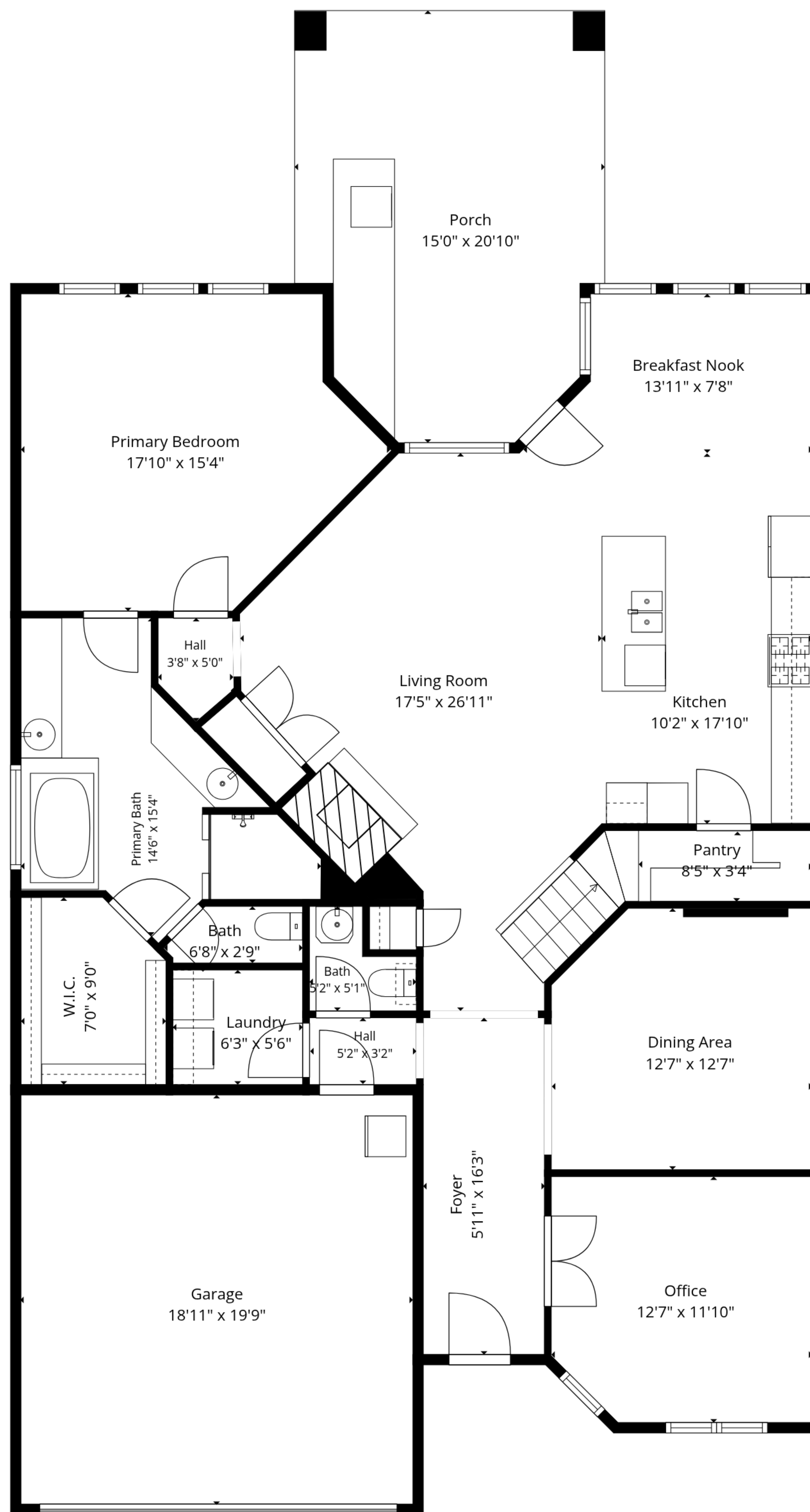
1st Floor
