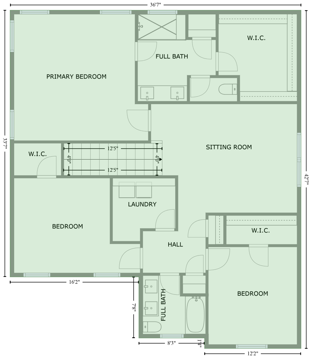
FLOOR 2 [AREA: 1401]
