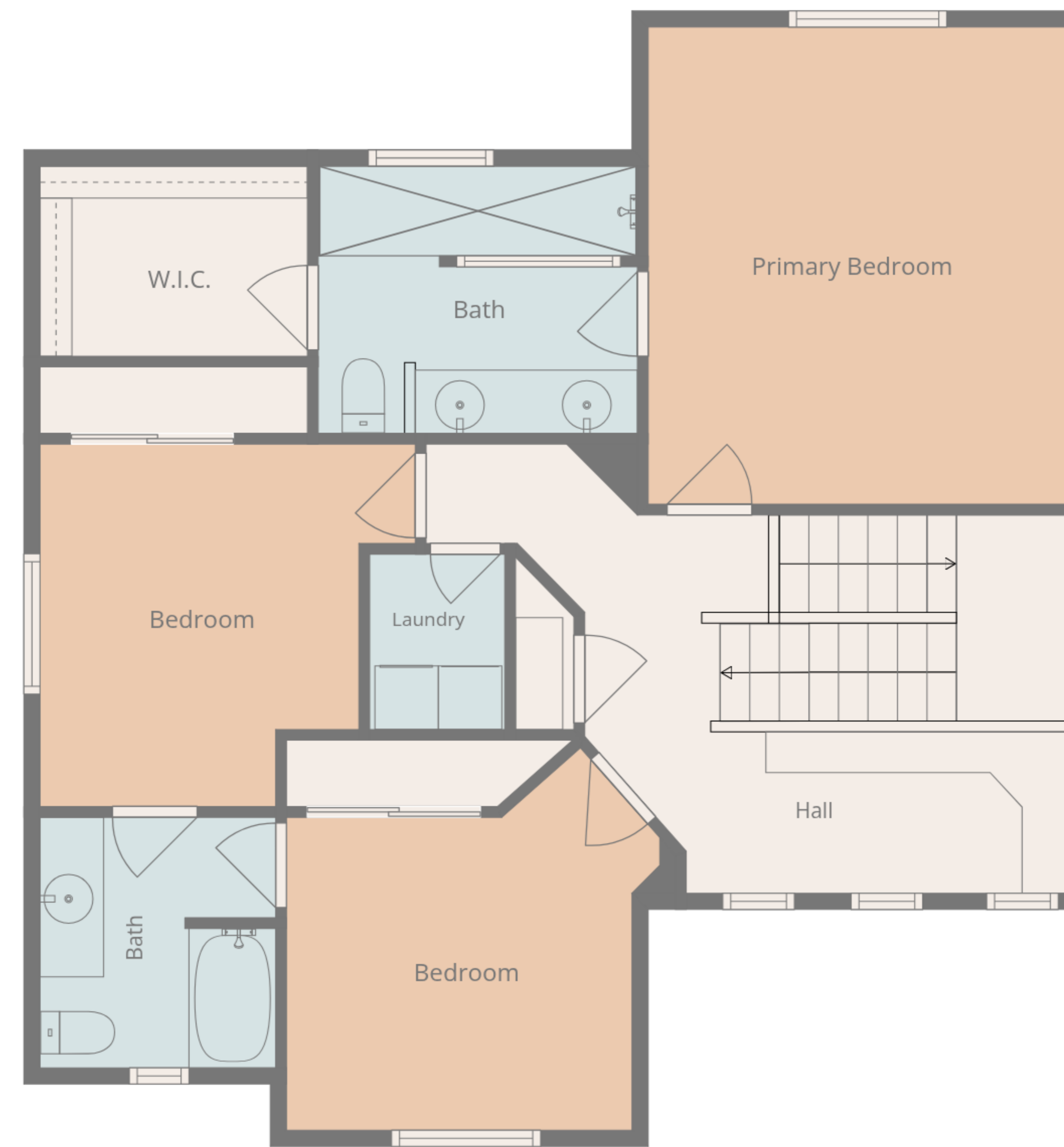
2nd Floor
