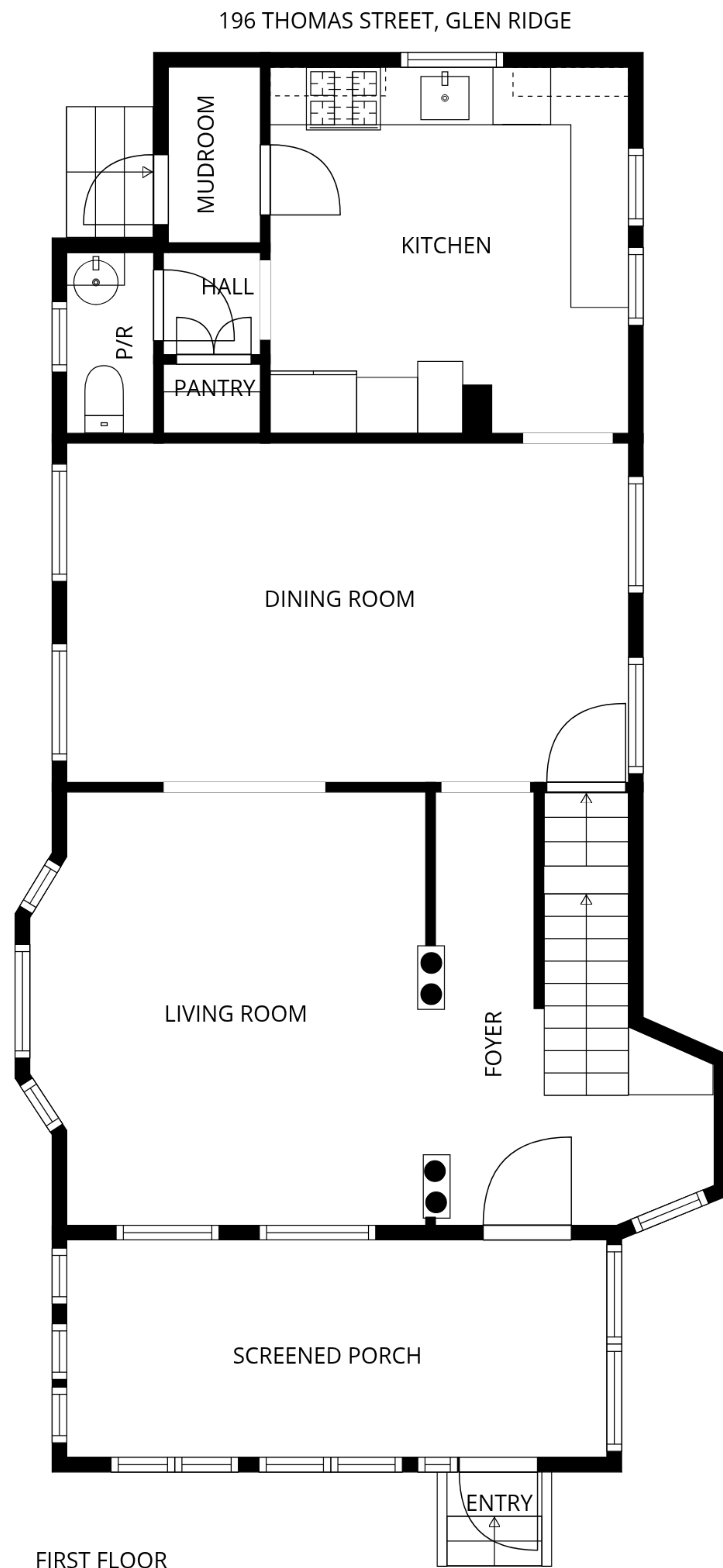
FIRST FLOOR
