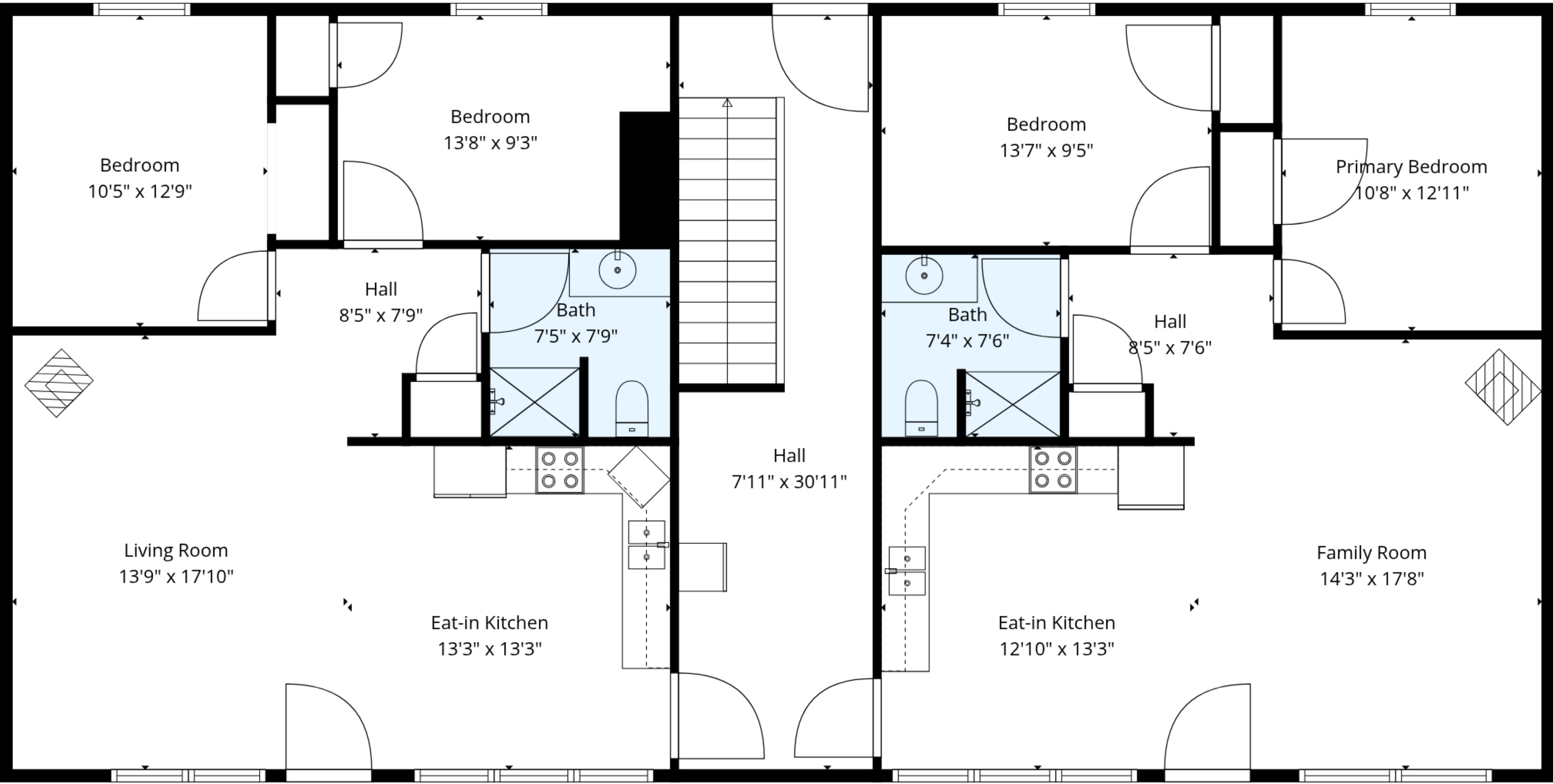
2nd Floor
