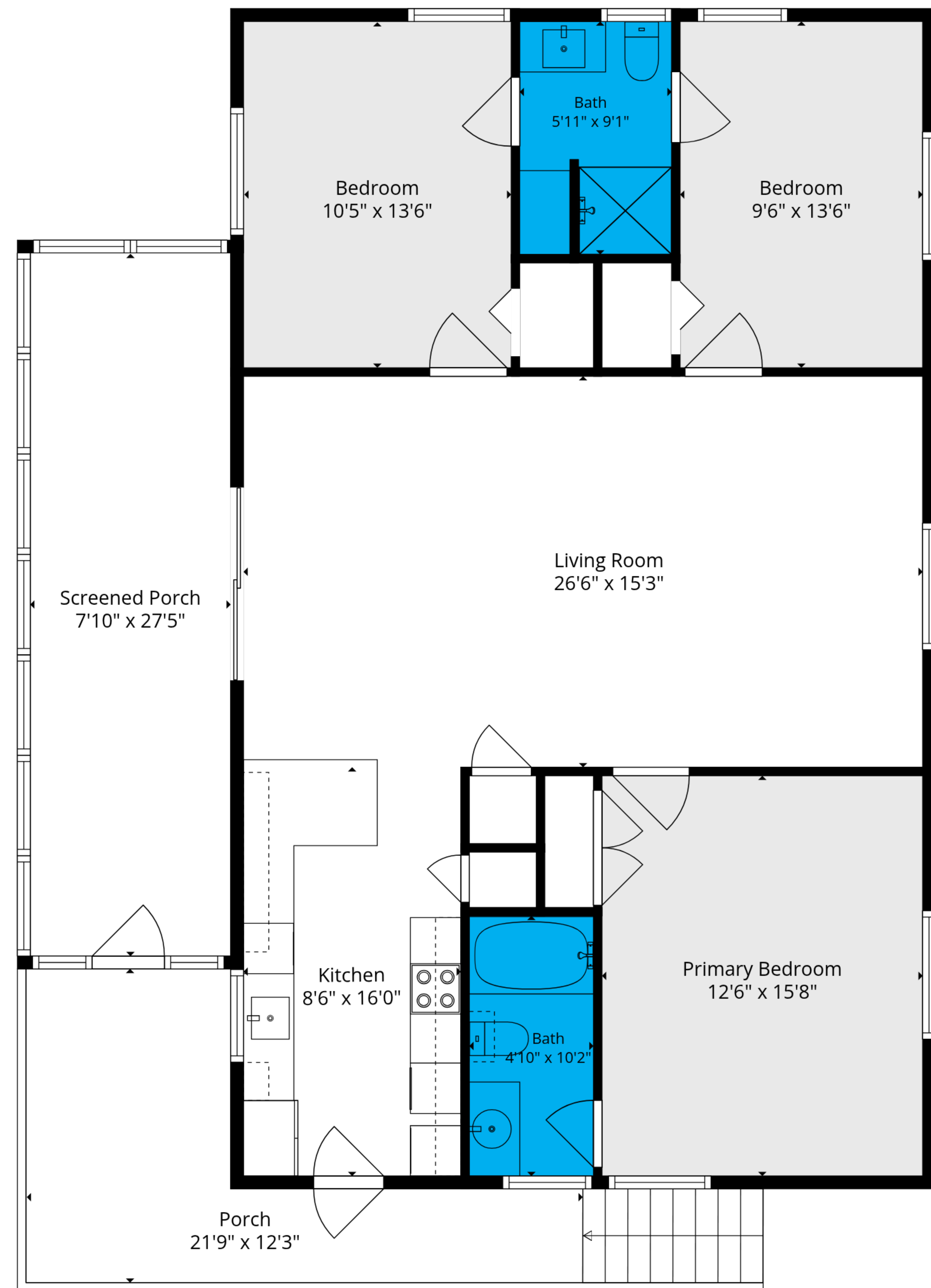
1st Floor
