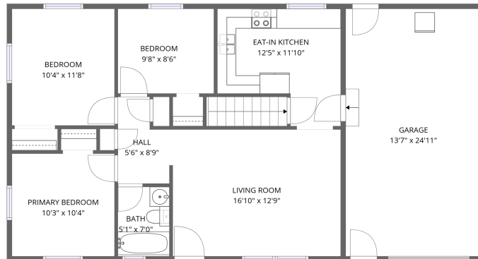
1st floor
