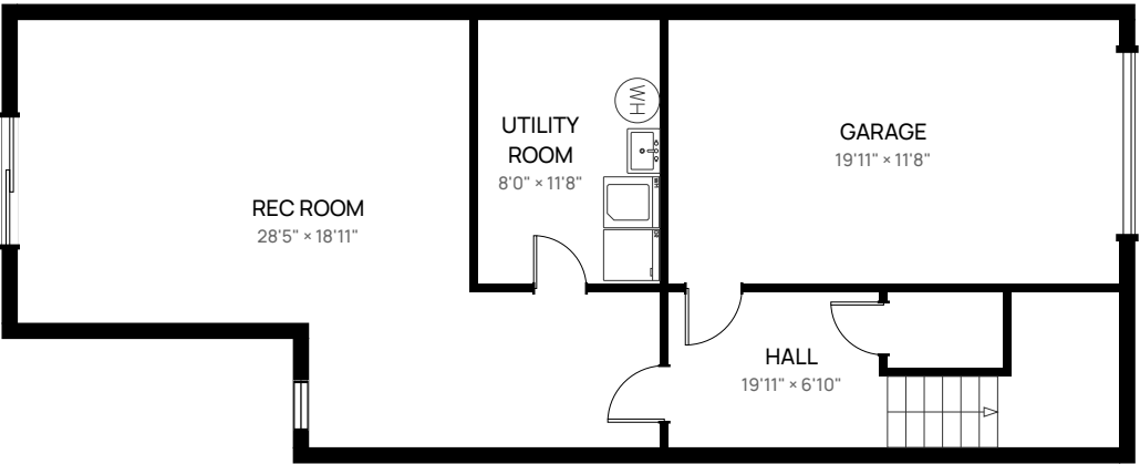
Basement
