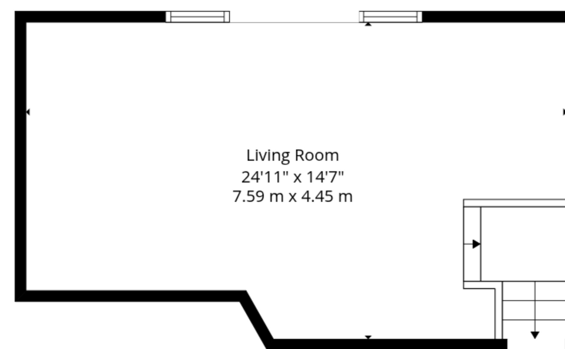
2nd Floor
