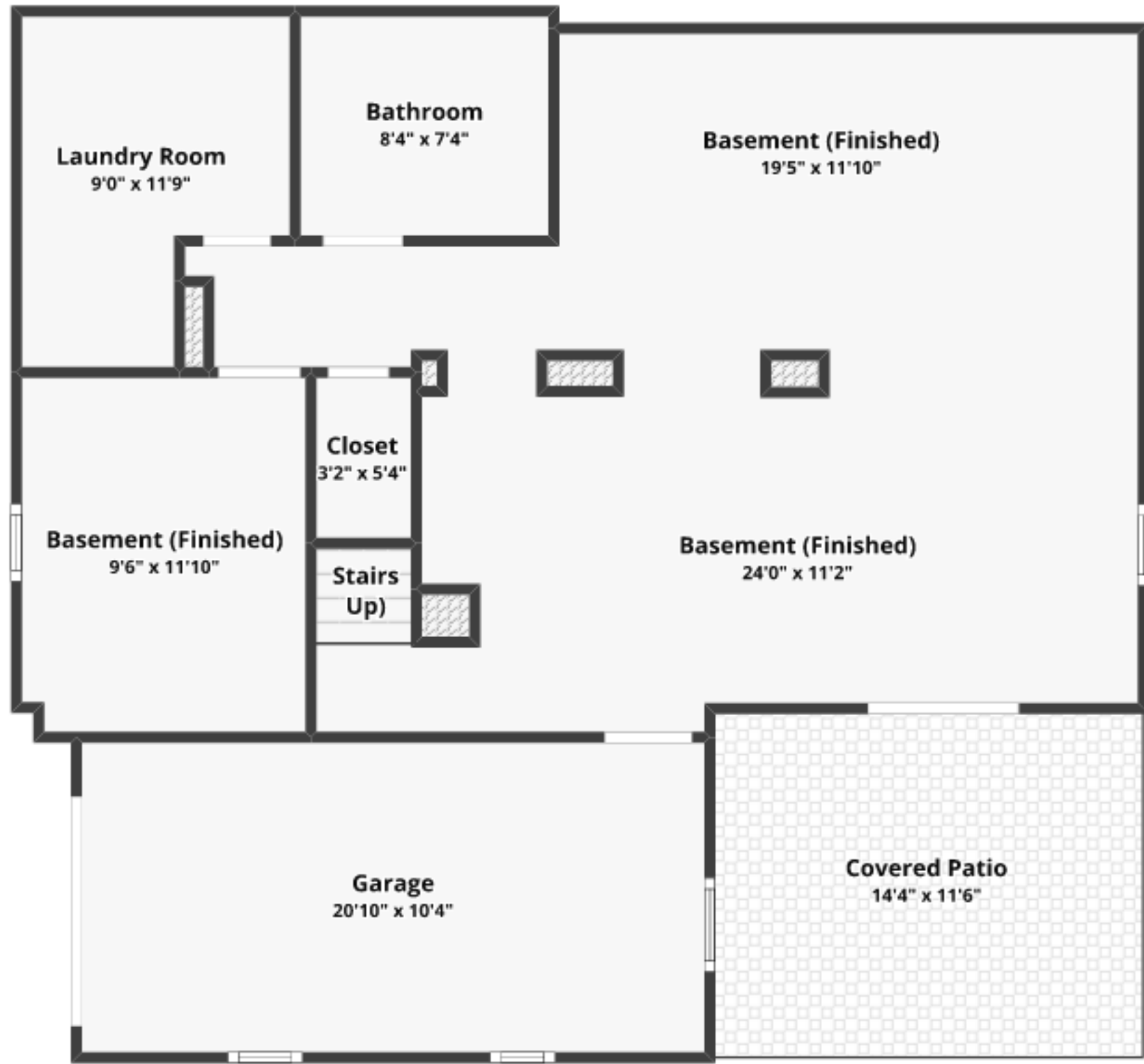
BASEMENT Finished area: ~824.09 sq. ft.
