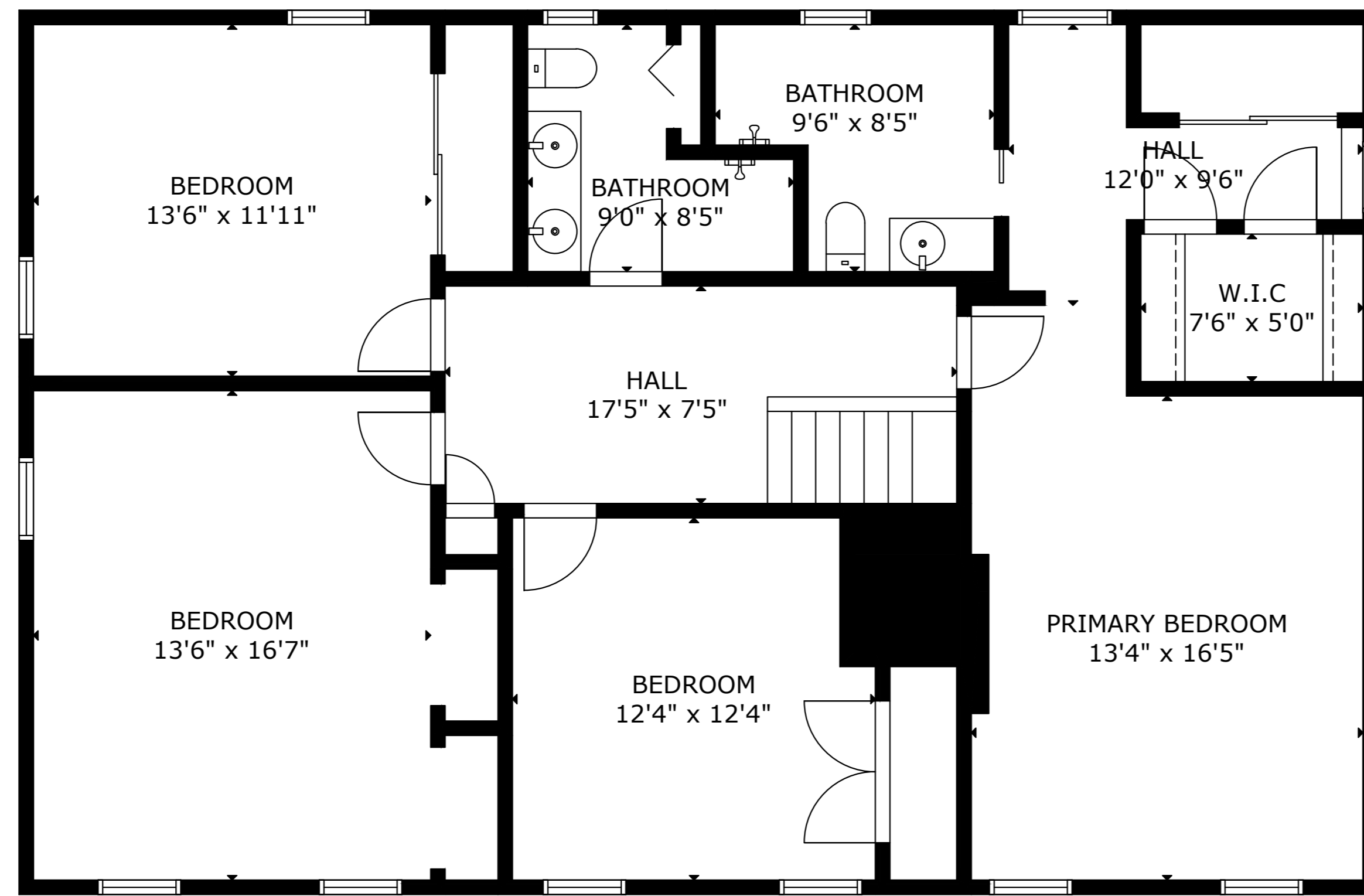
SECOND FLOOR
