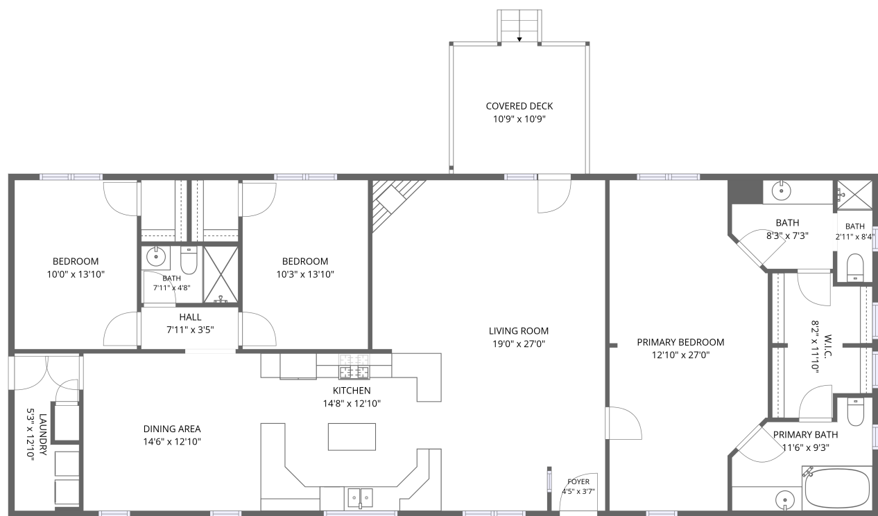
1st floor
