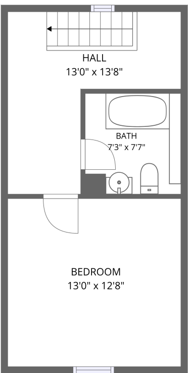
2nd floor
