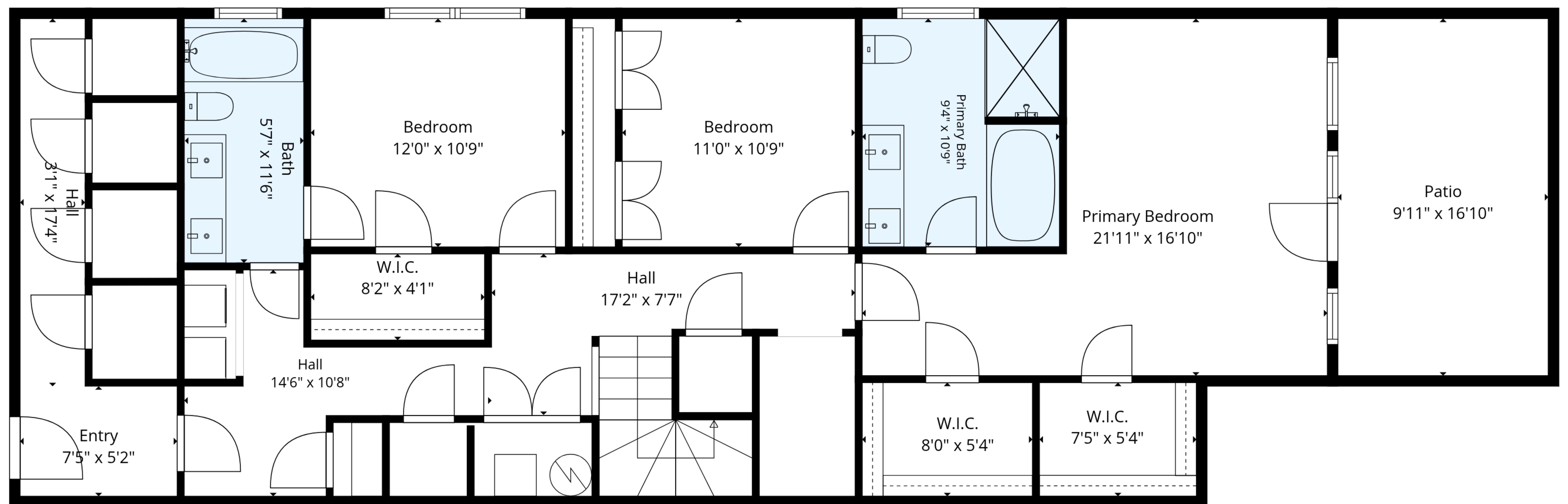
1st Floor
