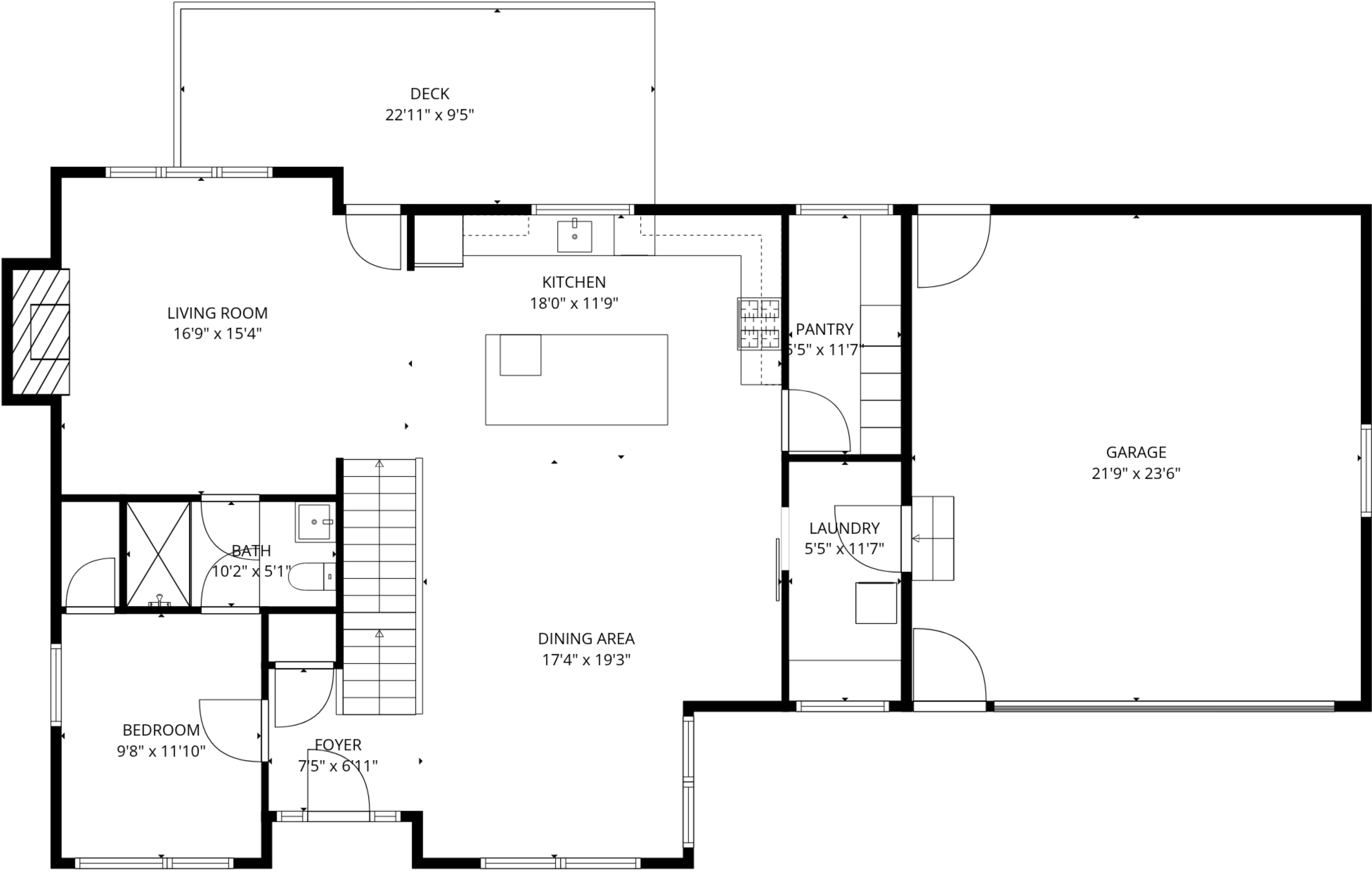
1st floor
