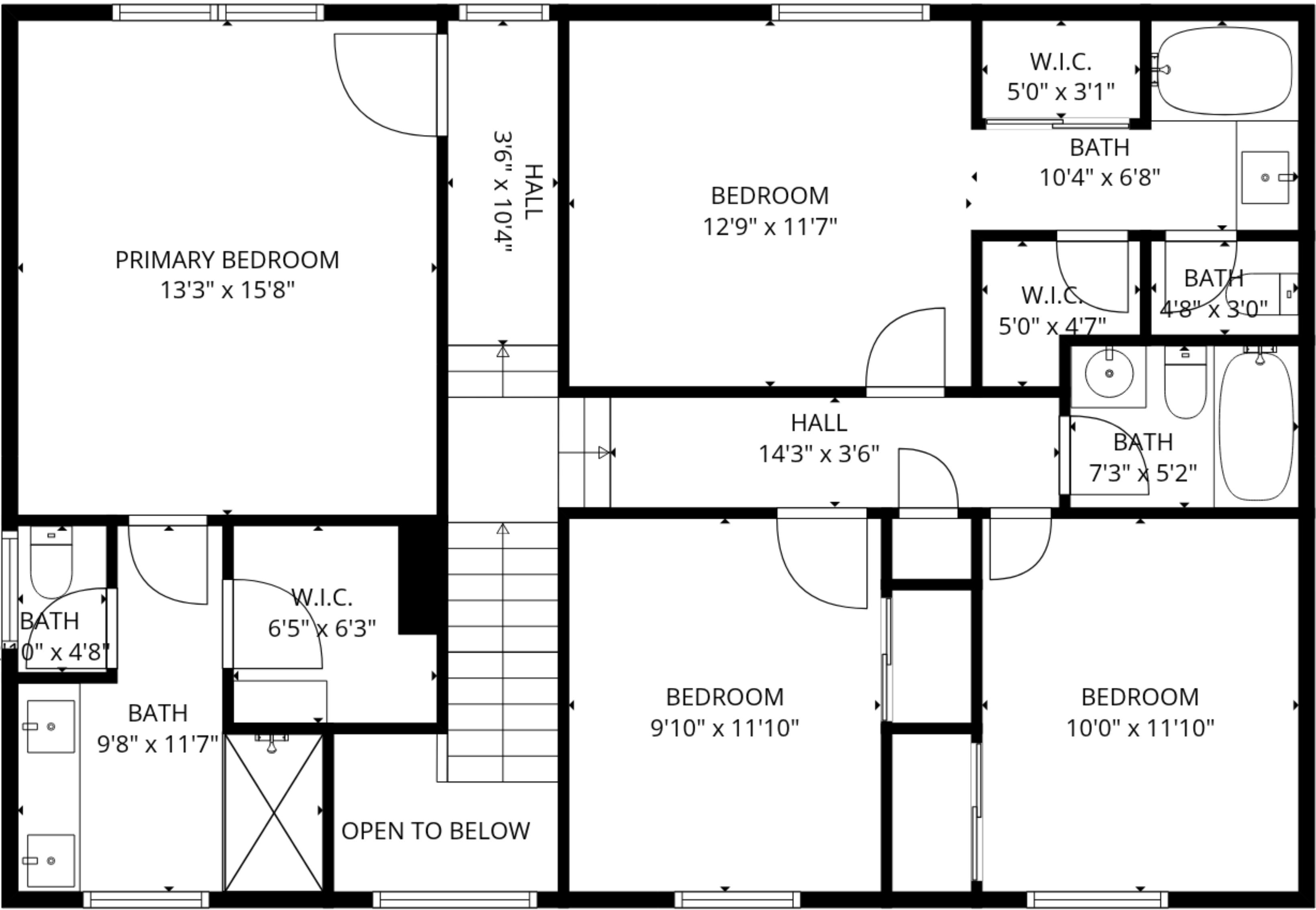
2nd floor
