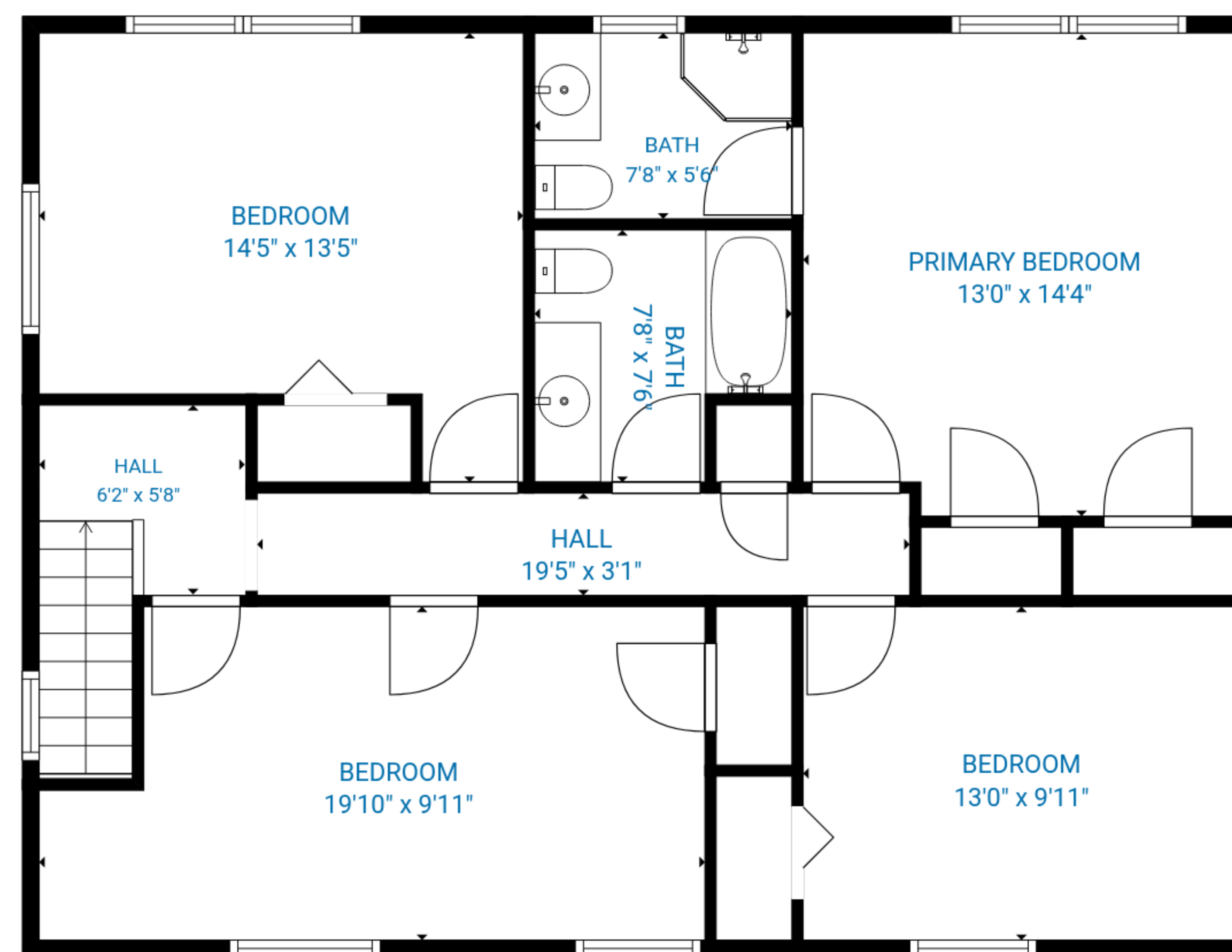
2nd floor
