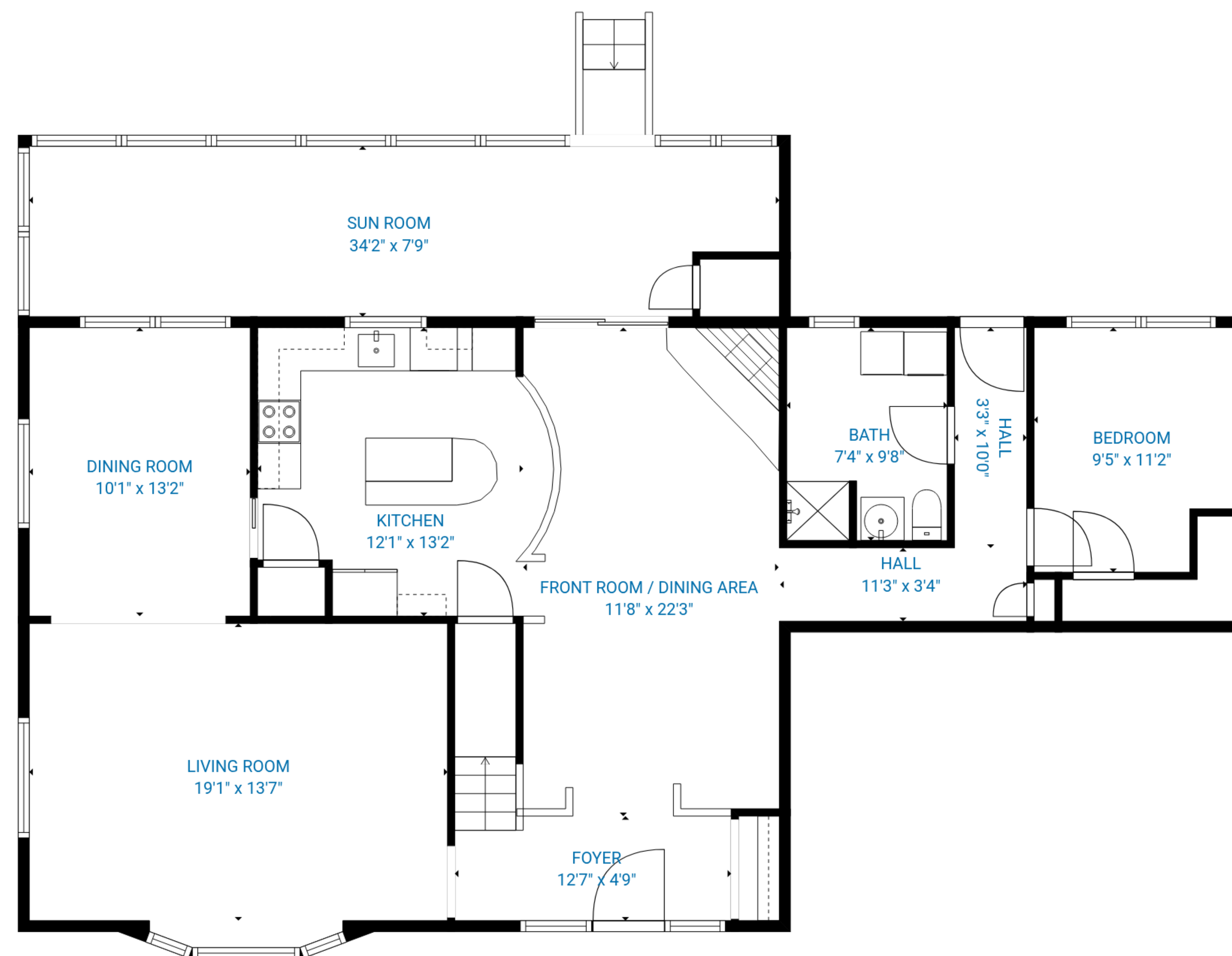
1st floor
