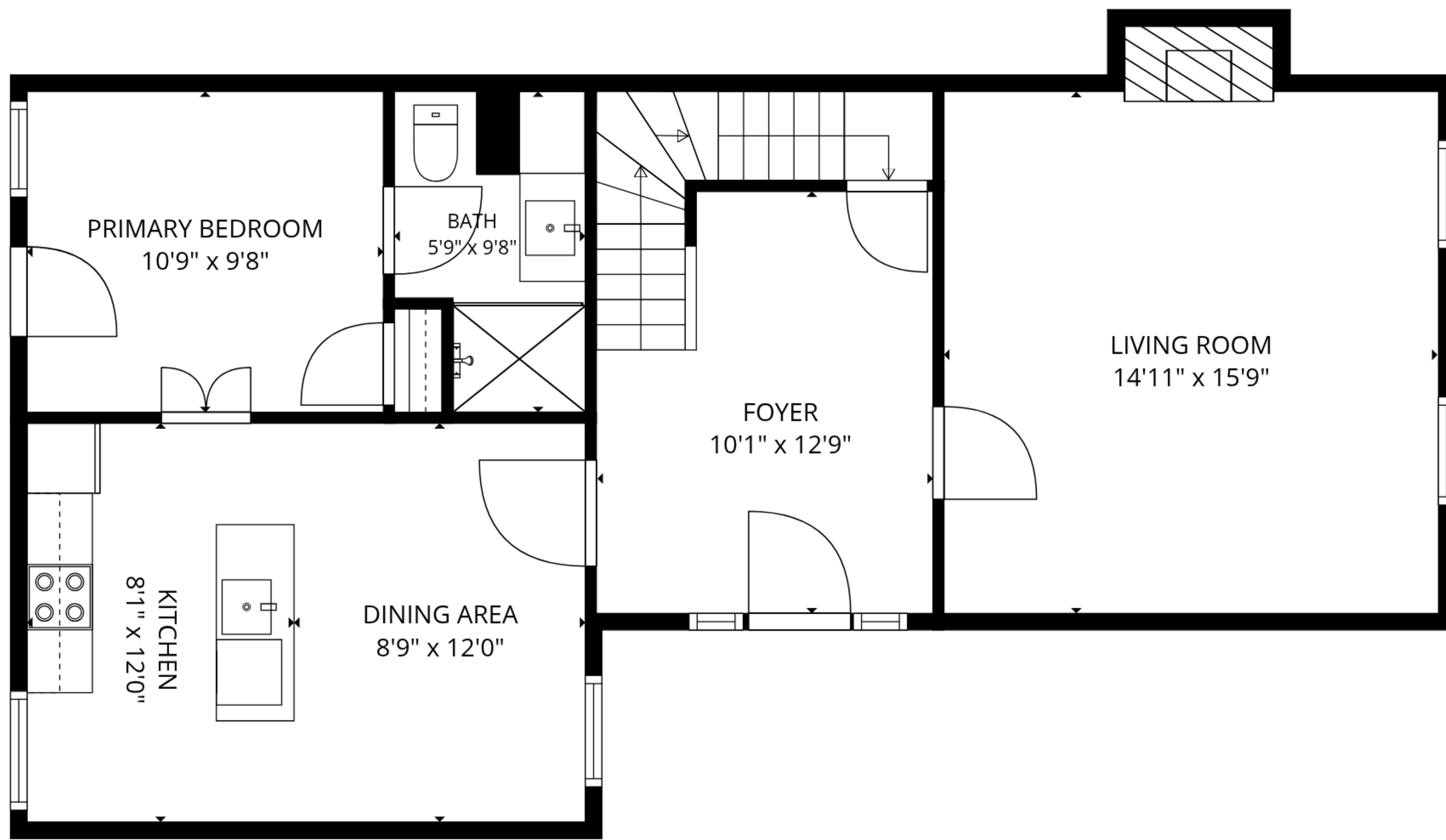
1st floor
