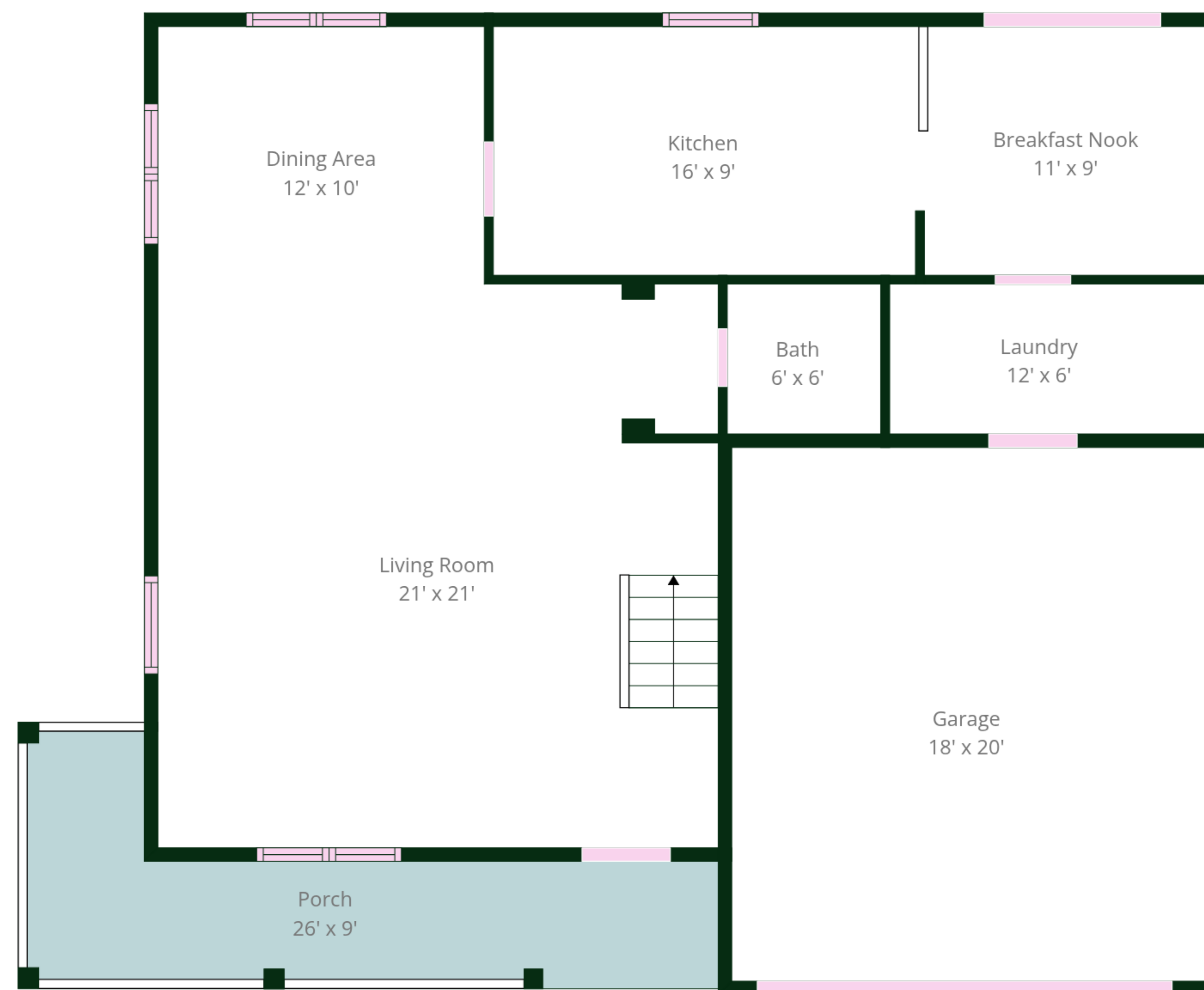
1st Floor
