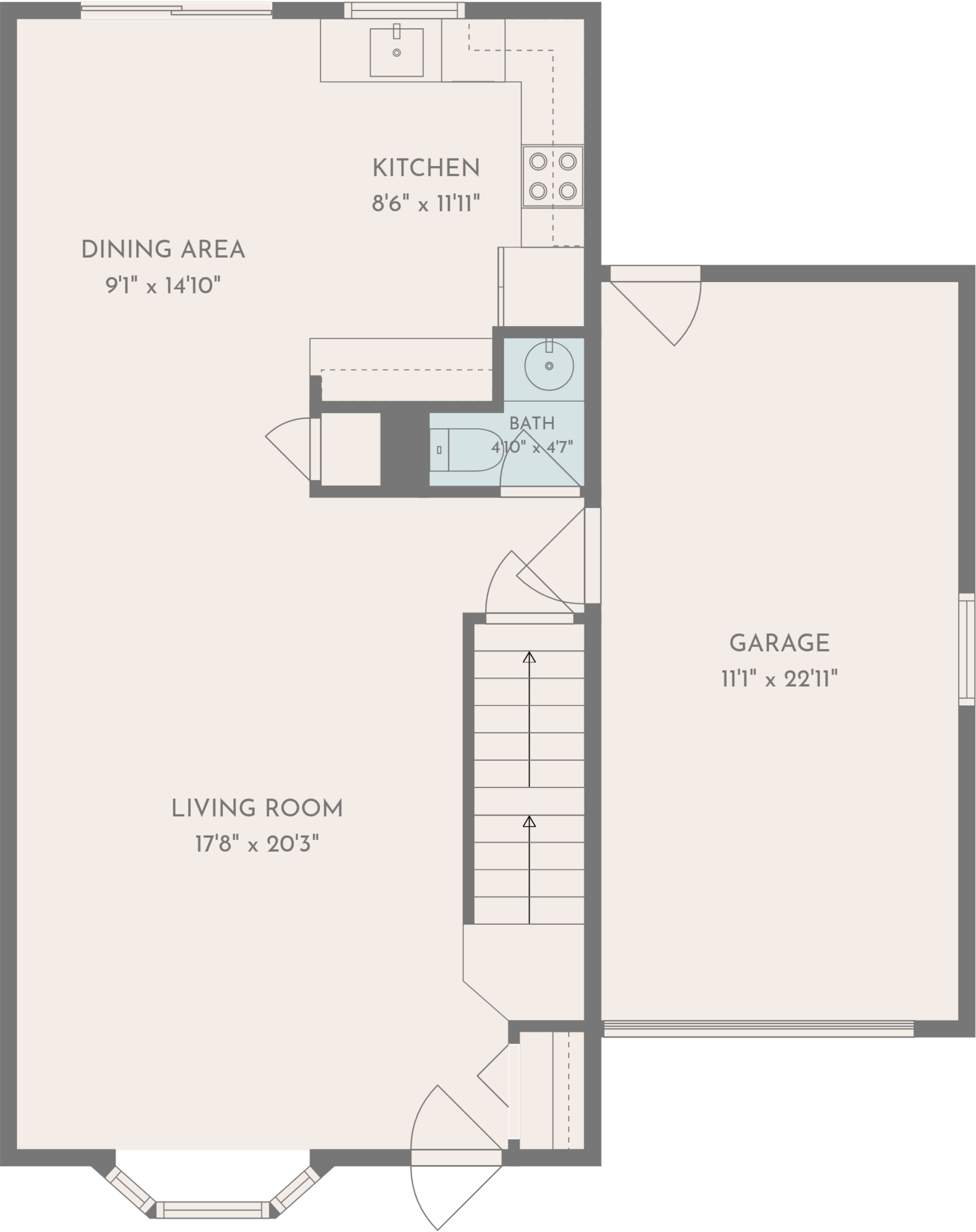
1st floor
