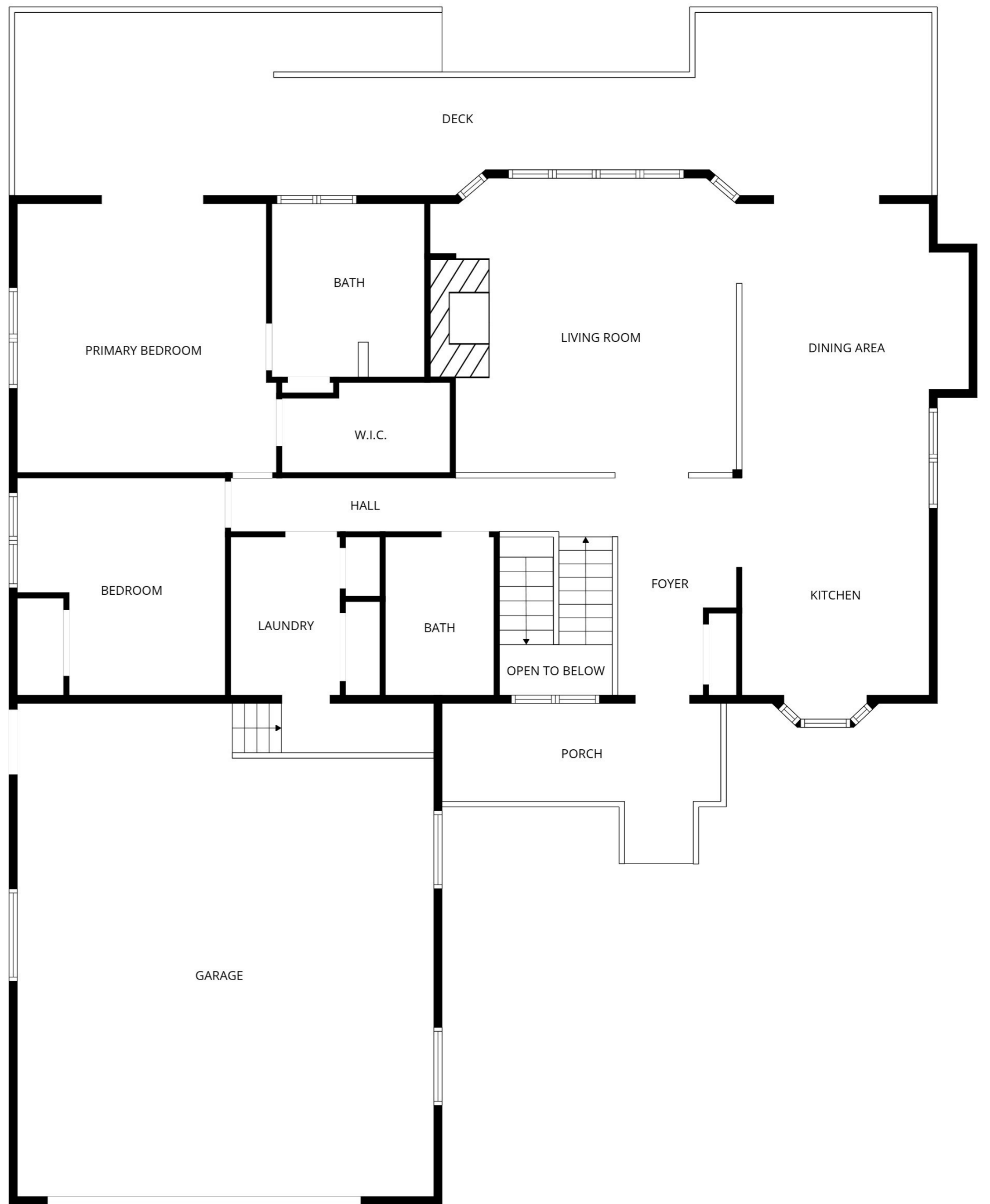
1st floor
