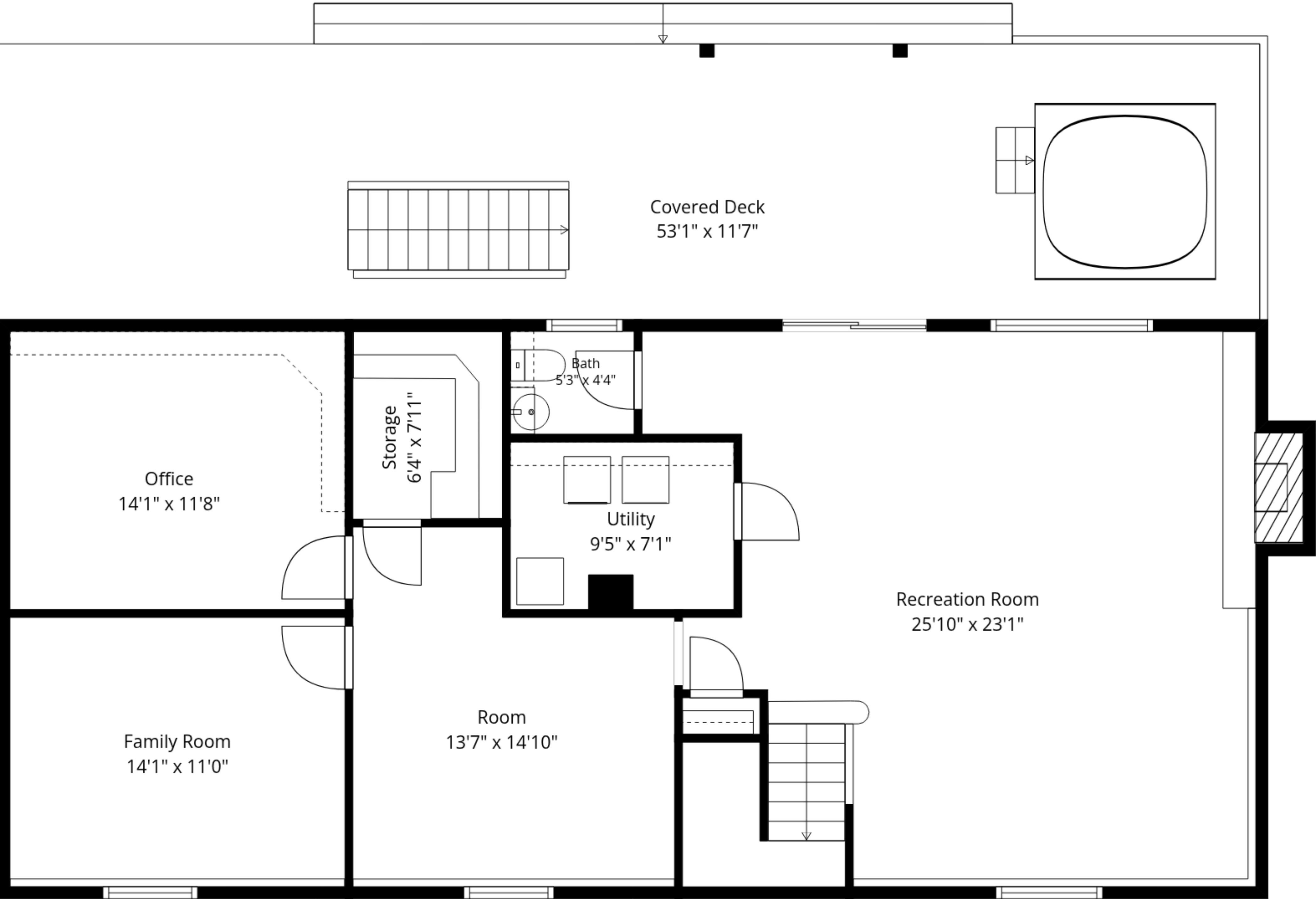
2nd Floor
