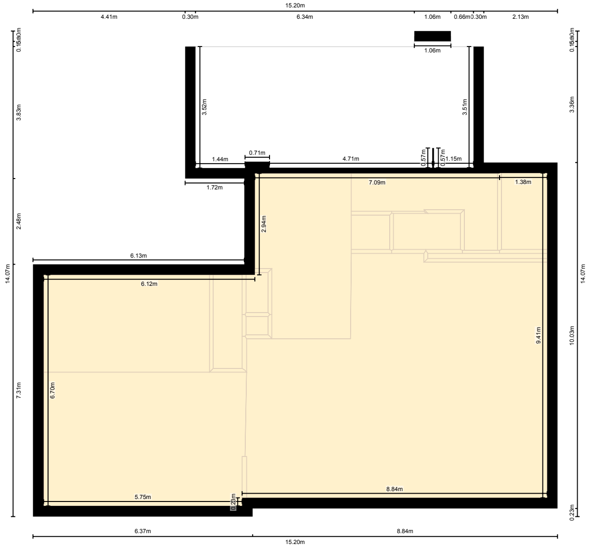
Measurement Diagram for: Main Floor Exterior Wall Thickness: 31 cm
