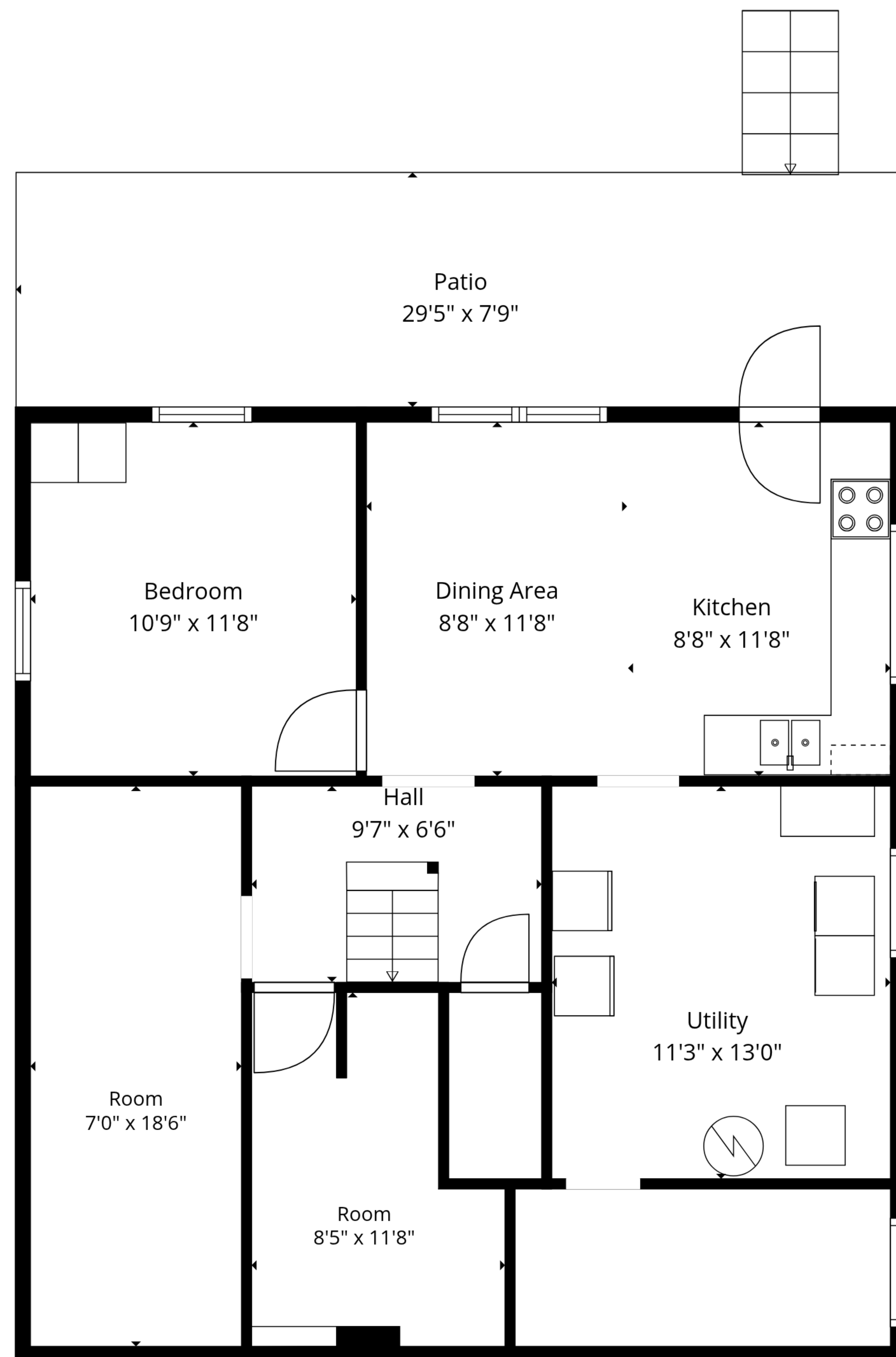
Basement
