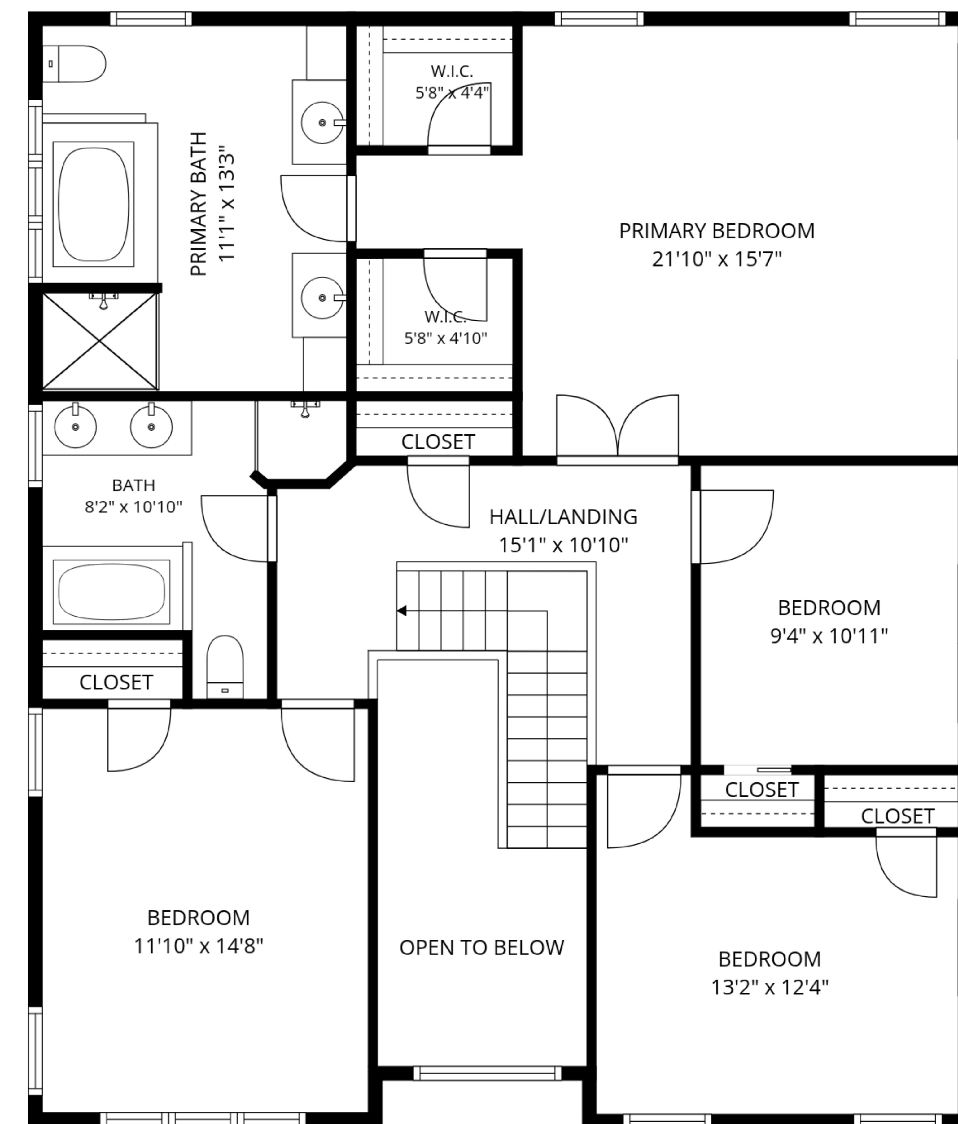
2nd floor
