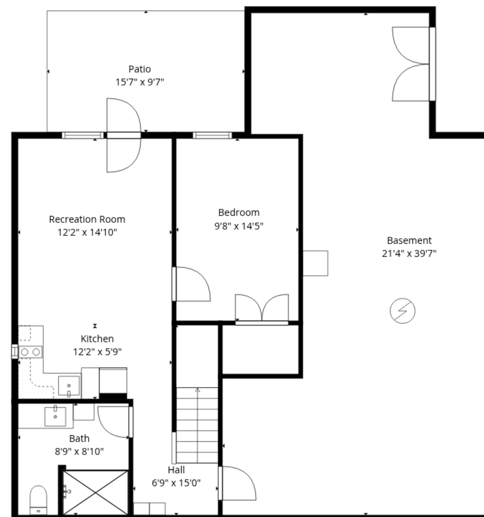
Basement 1
