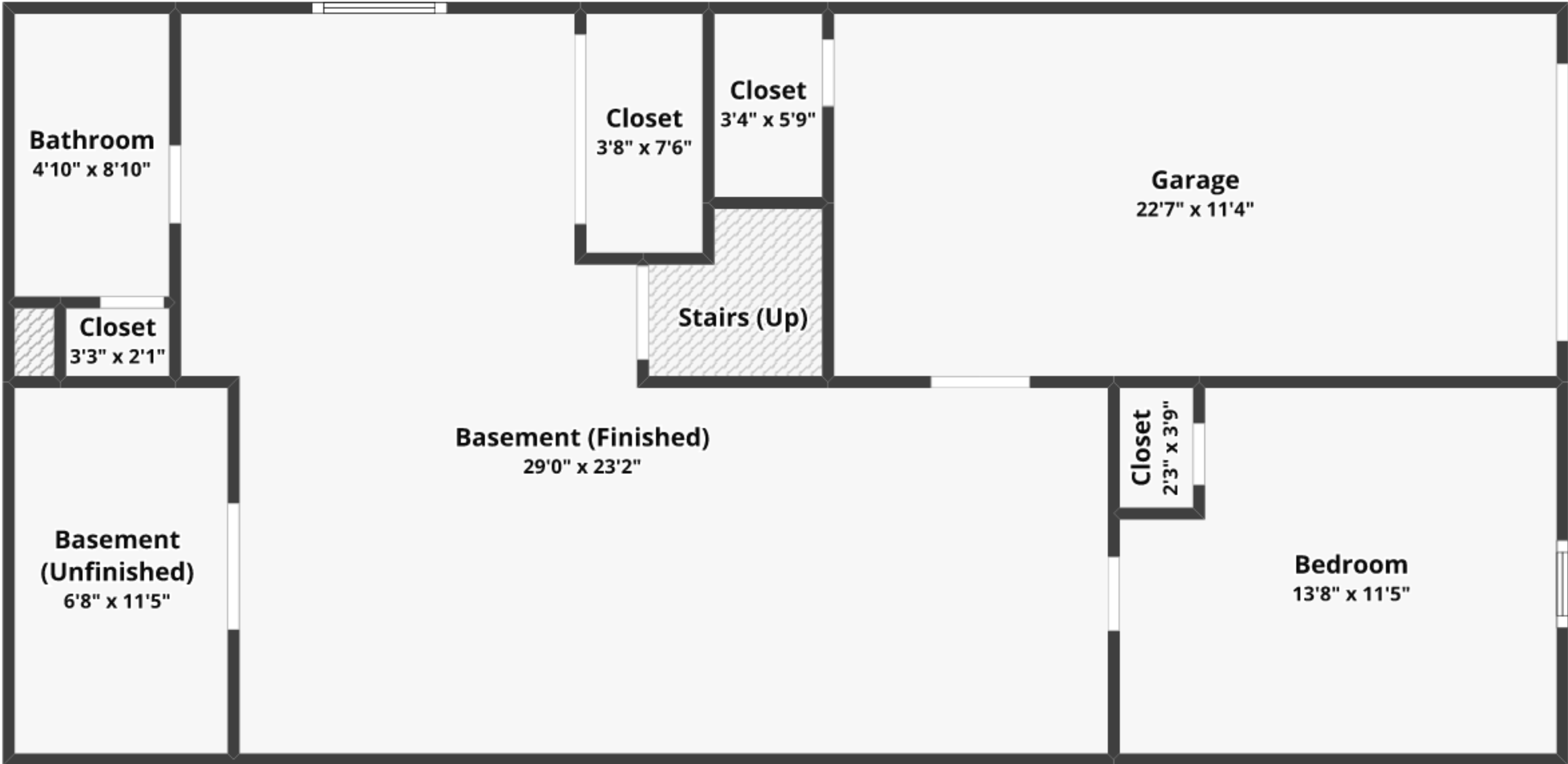
BASEMENT Finished area: ~691.13 sq. ft. Unfinished area: ~78.72 sq. ft.
