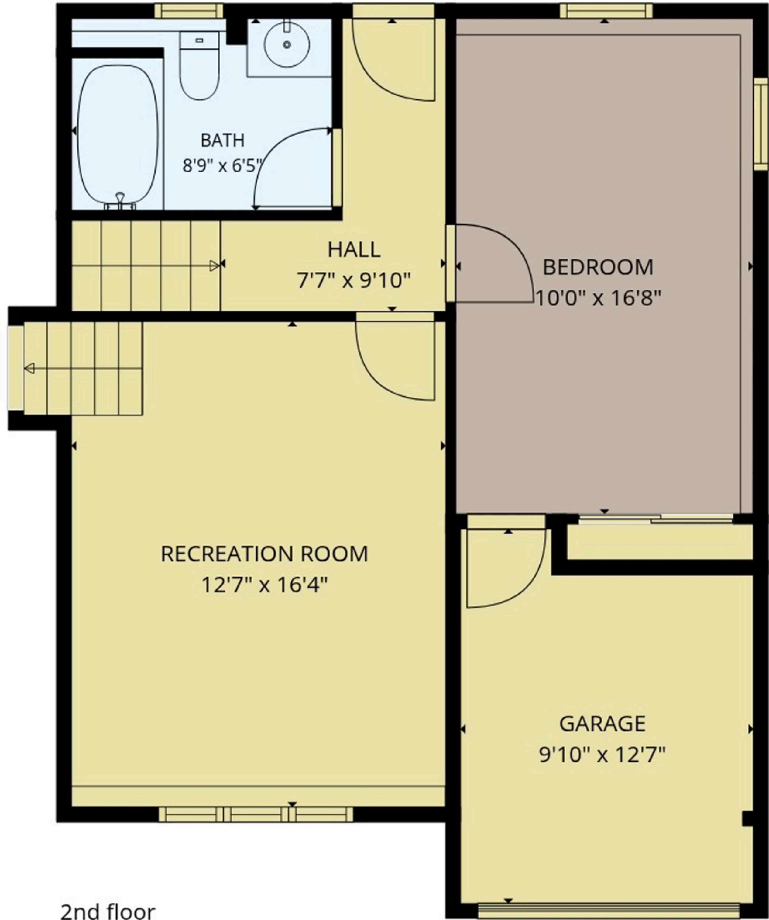
2nd floor
