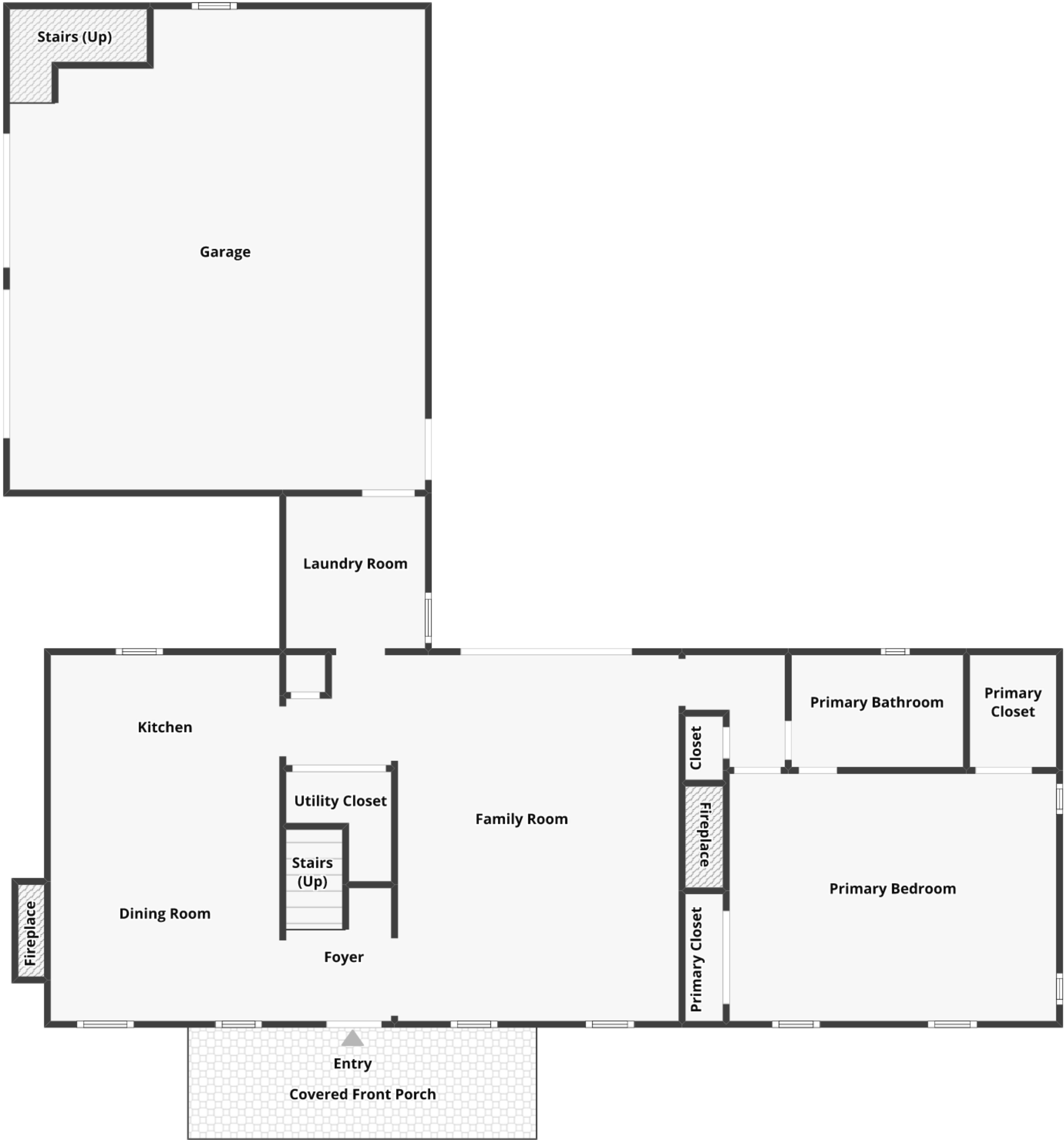
FLOOR 1
