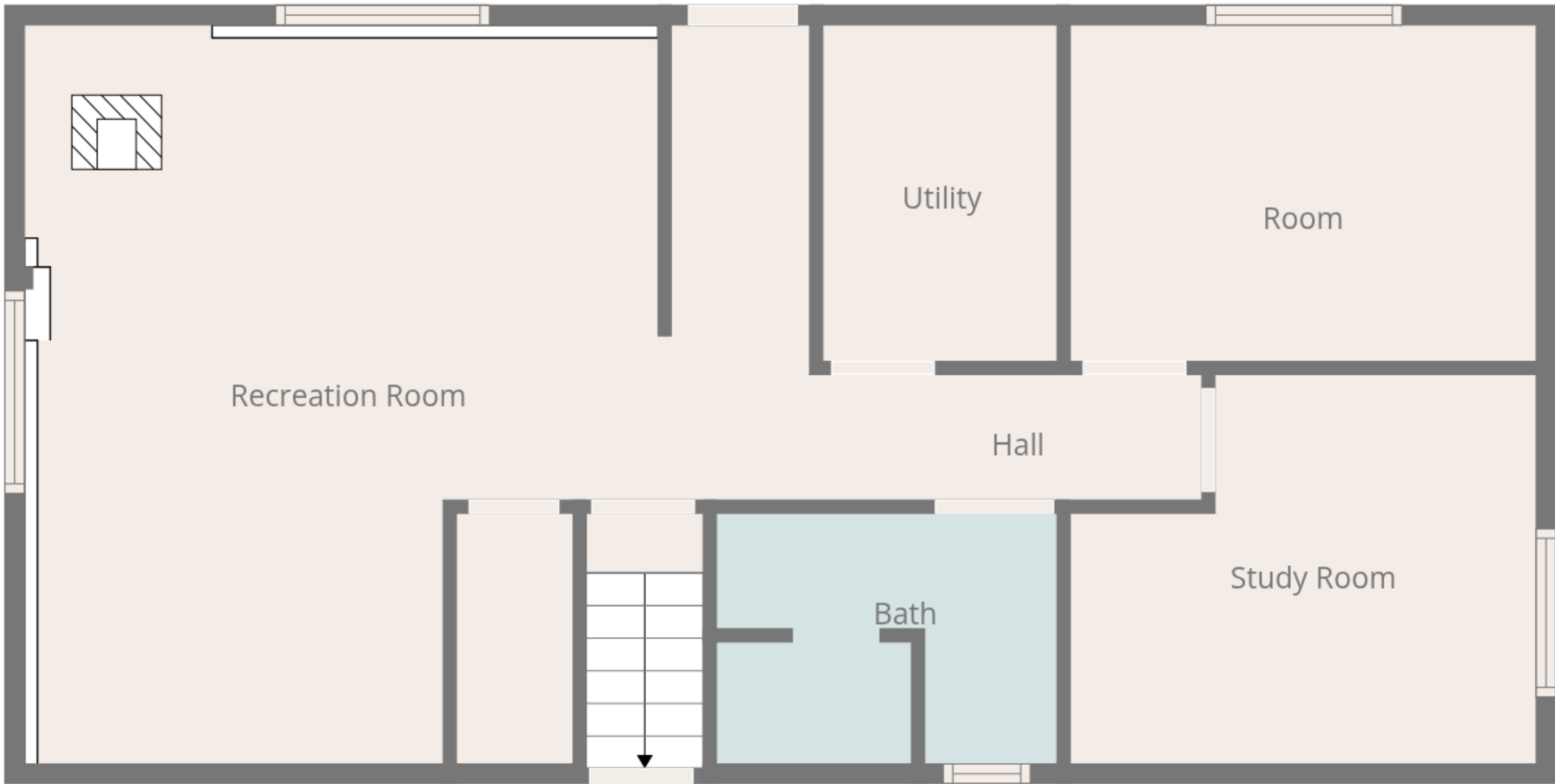
1st Floor
