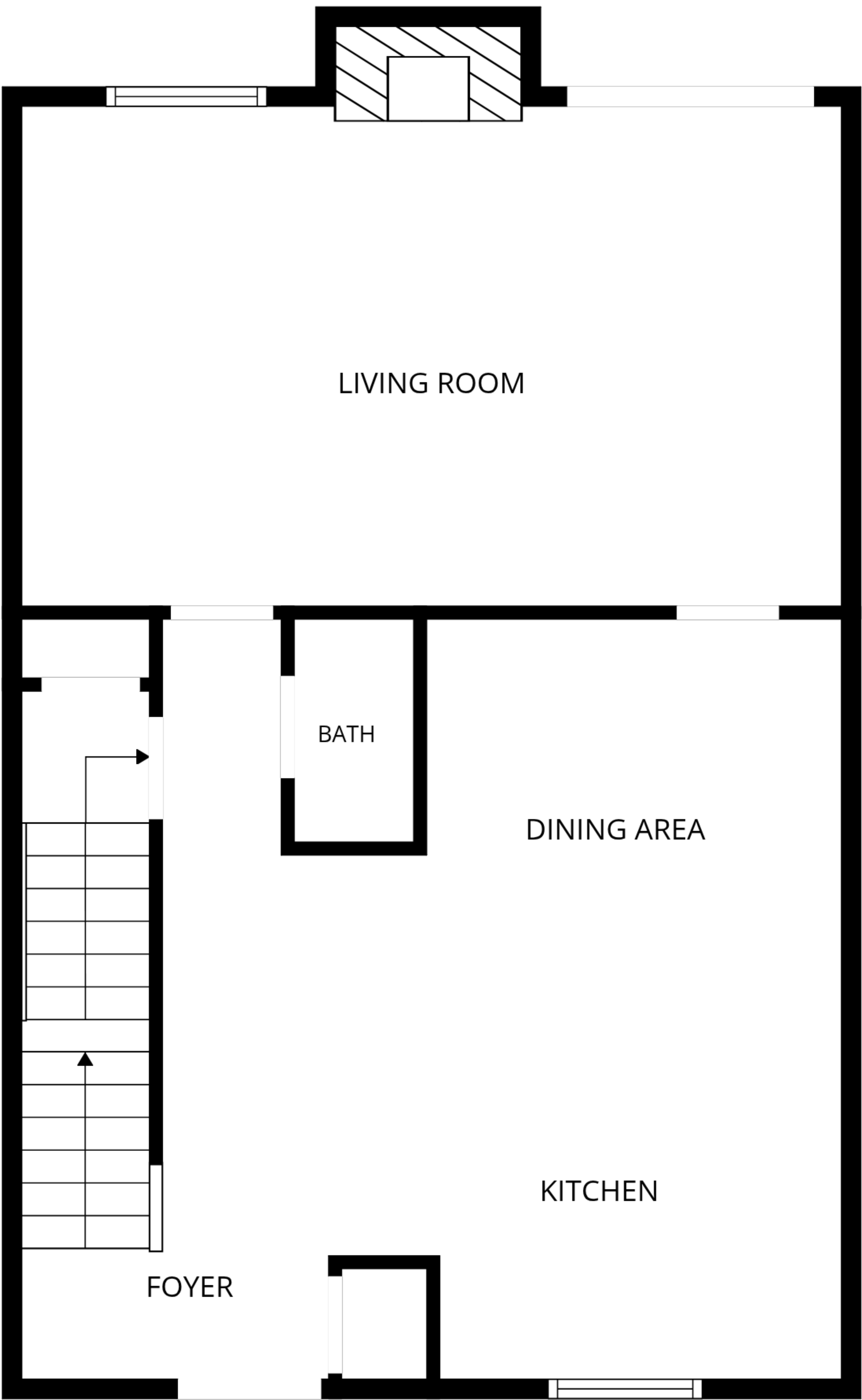
2nd floor
