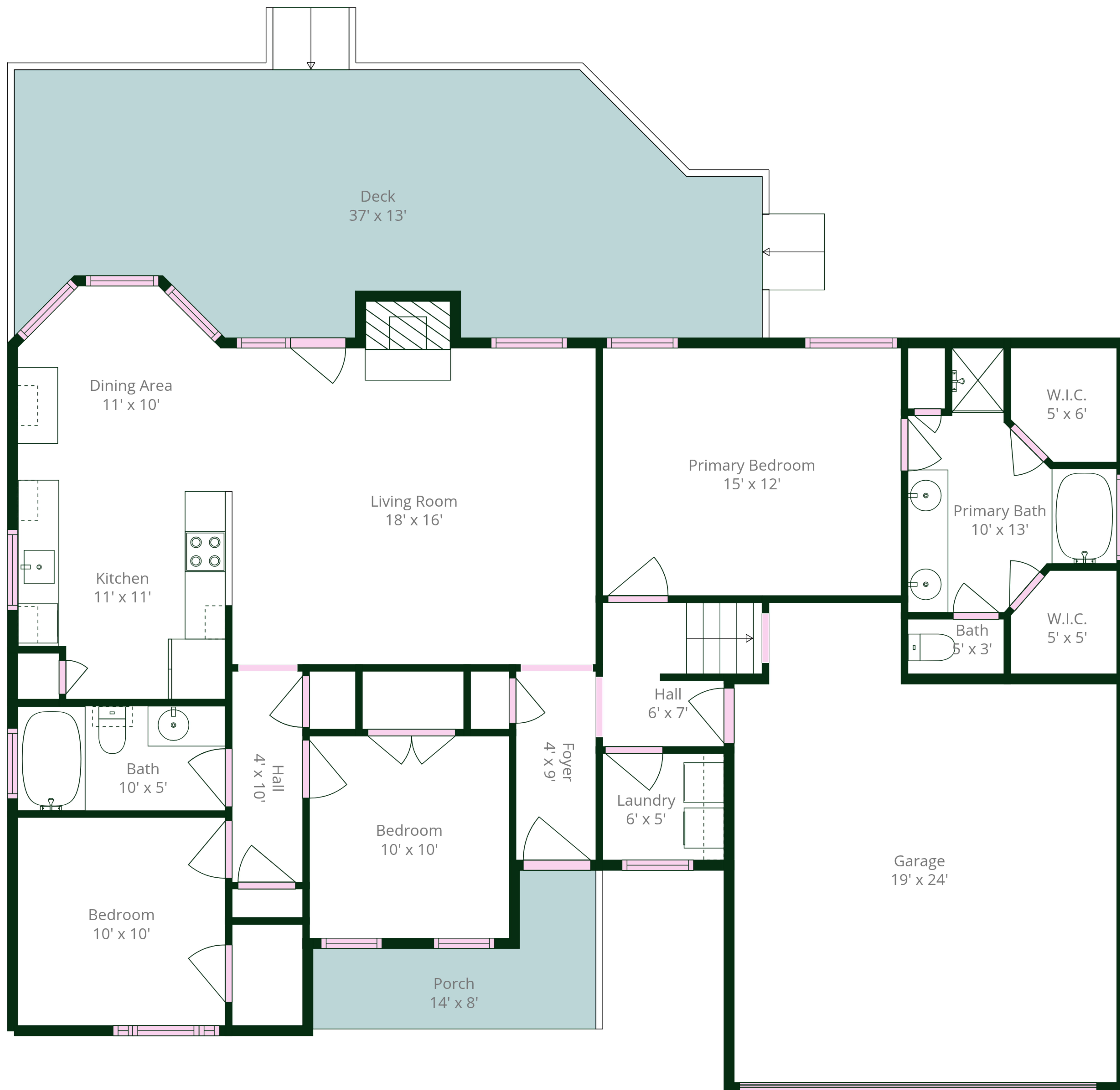
Floor 1
