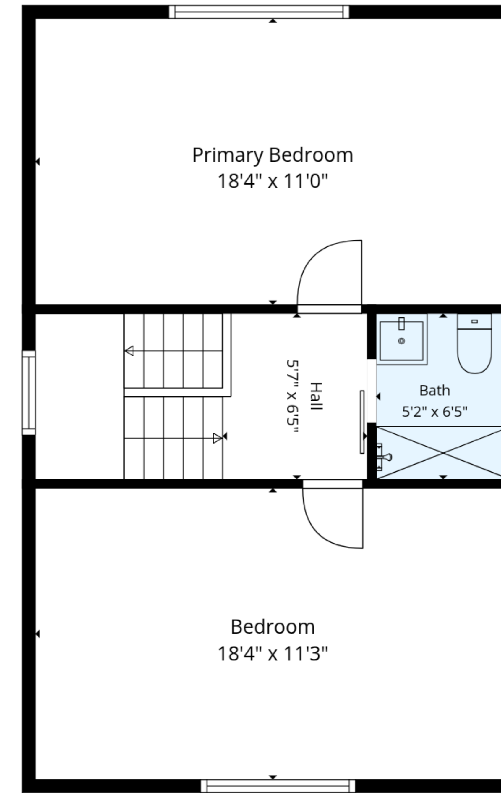
1st Floor
