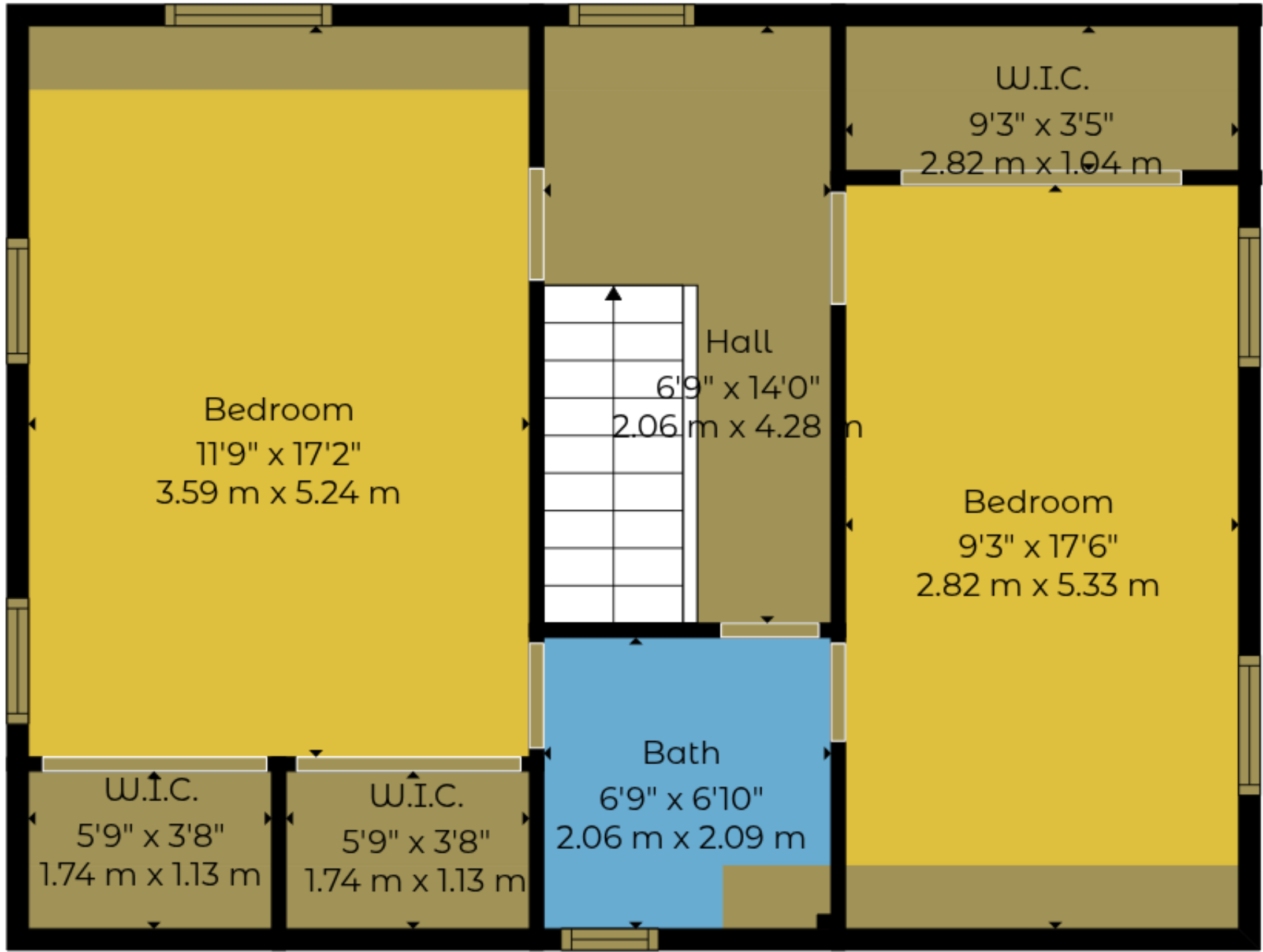
2nd Floor
