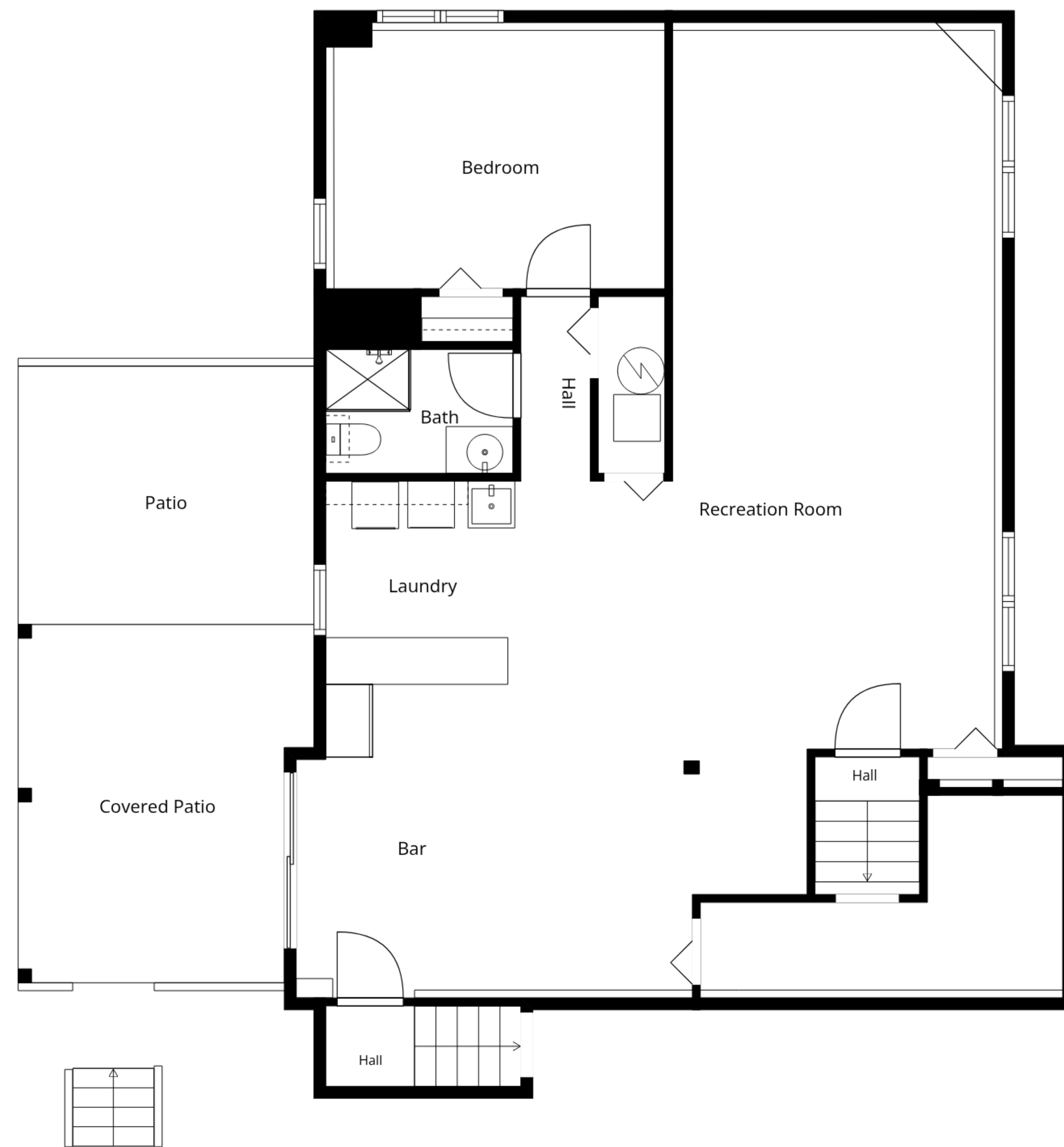
1st Floor
