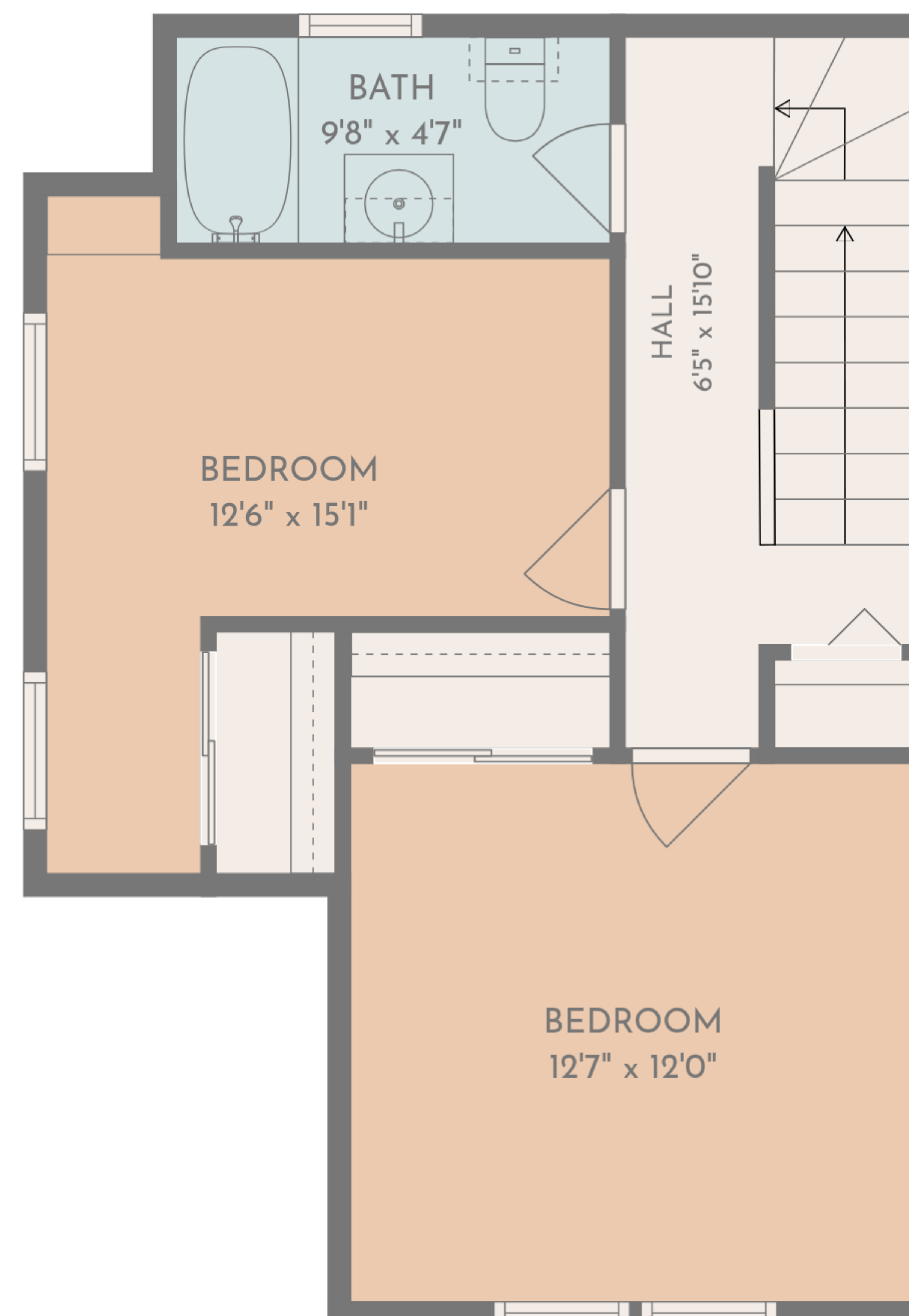
2nd floor
