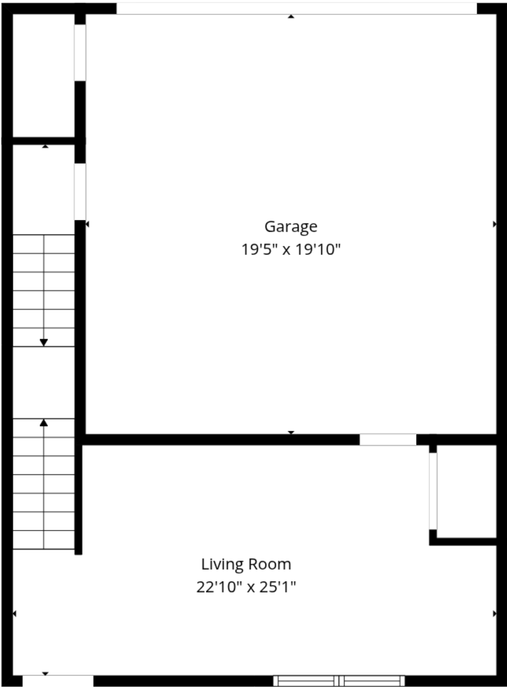
Ground Floor
